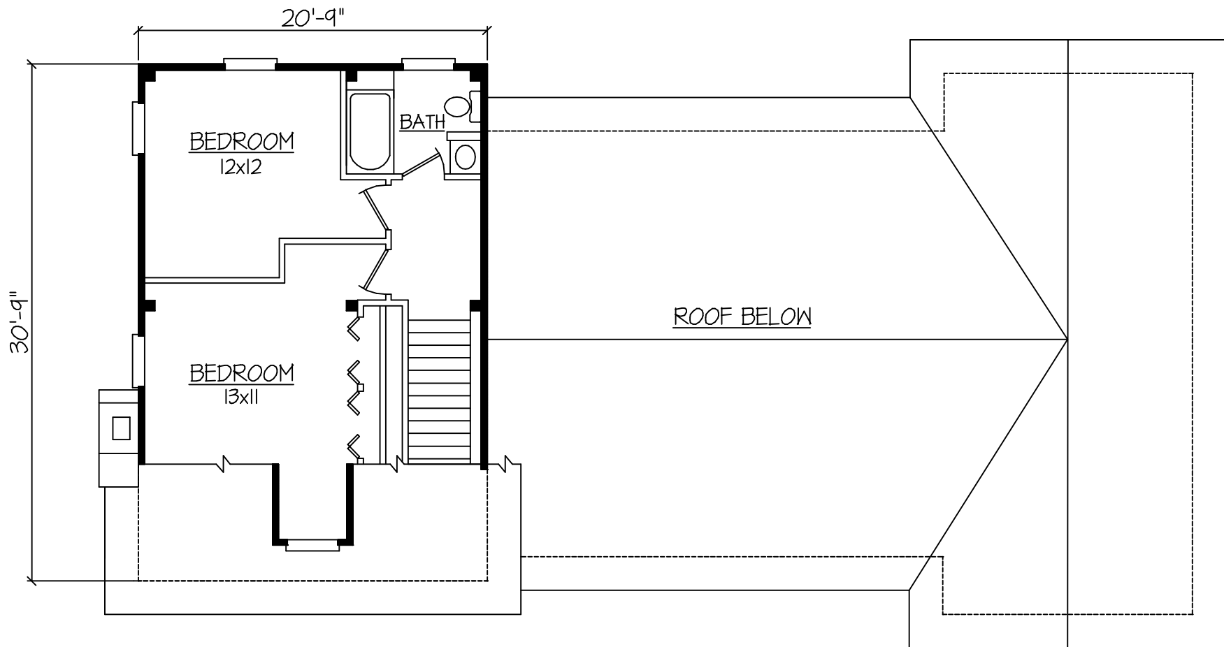
SECOND FLOOR PLAN SECOND FLOOR - 540 SF
