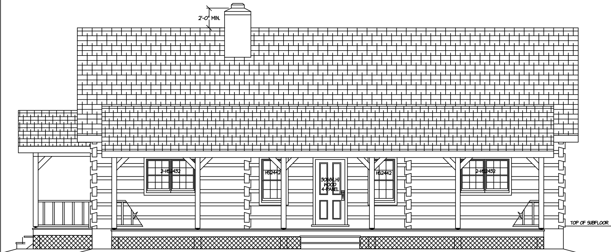
PLAN FRONT
