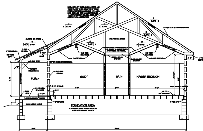
SECTION THRU STUDY/BATH/MASTER BEDROOM
