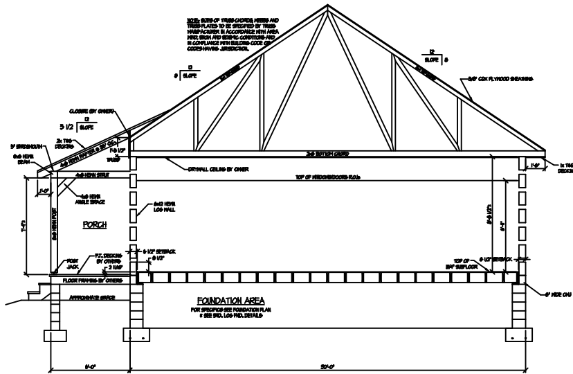
SECTION THRU BEDROOM/BATH/KITCHEN
