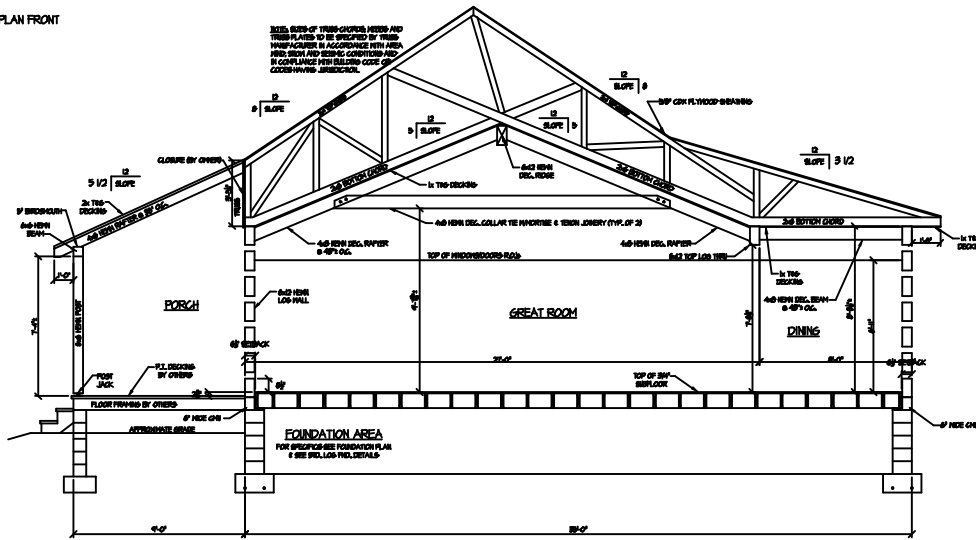
SECTION THRU GREAT ROOM/DINING
