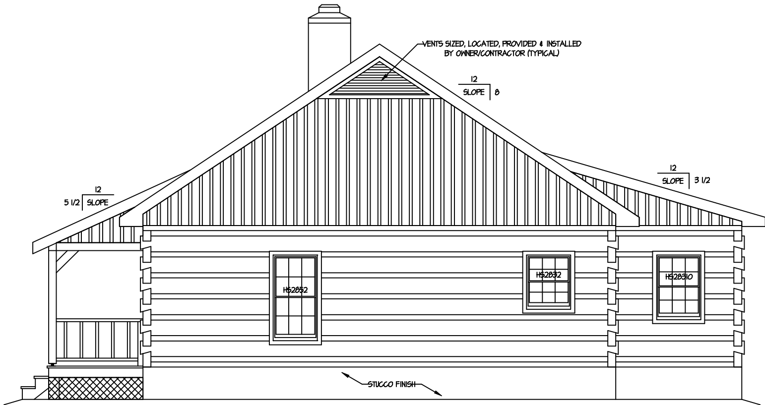
PLAN RIGHT
