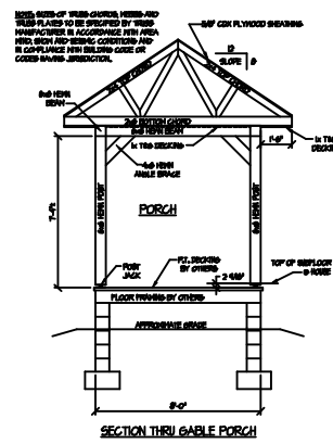
SECTION THRU GABLE PORCH
