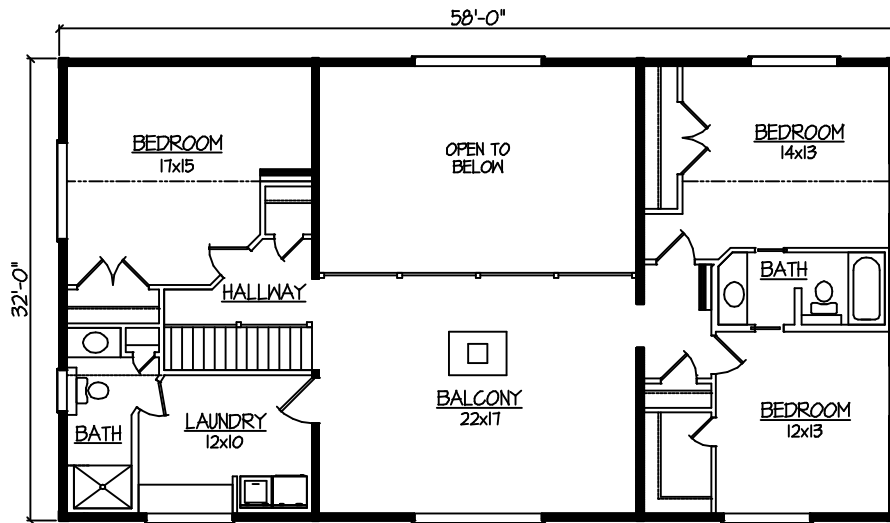
SECOND FLOOR PLAN SECOND FLOOR - 1530 SF
