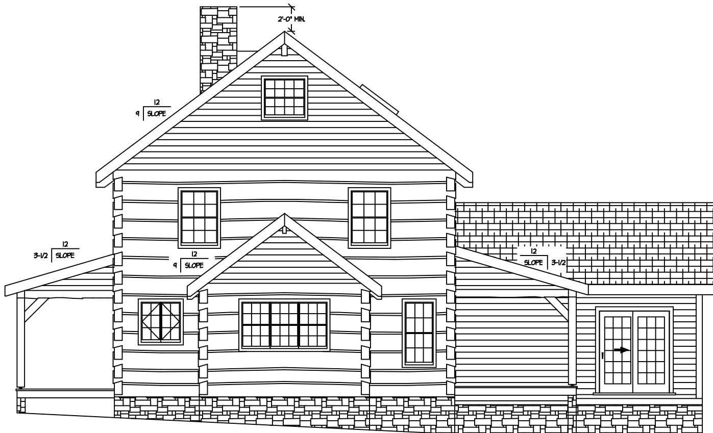
PLAN RIGHT ELEVATION
