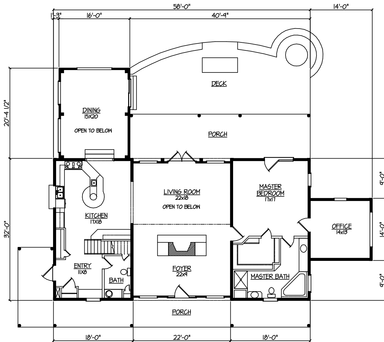
FIRST FLOOR PLAN FIRST FLOOR PLAN - 23185F TOTAL - 45035F
