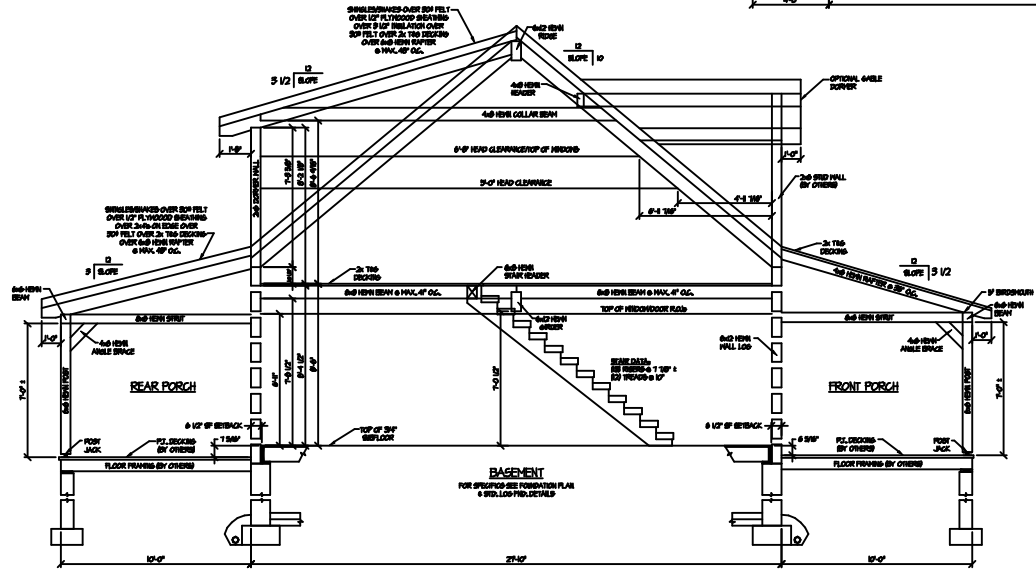
SECTION @ MASTER BEDROOM
