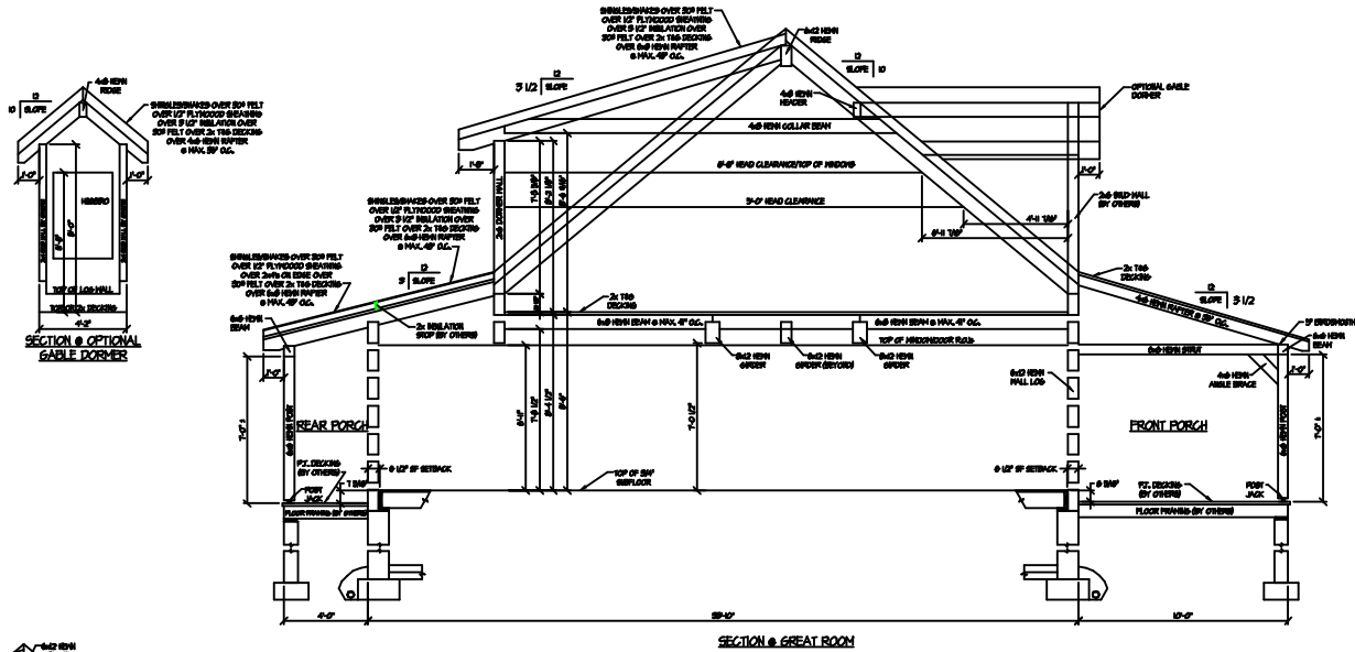
SECTION @ GREAT ROOM
