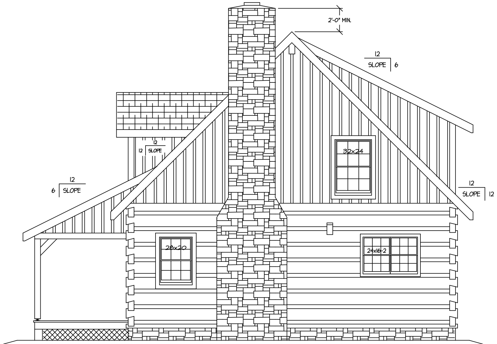
PLAN RIGHT ELEVATION
