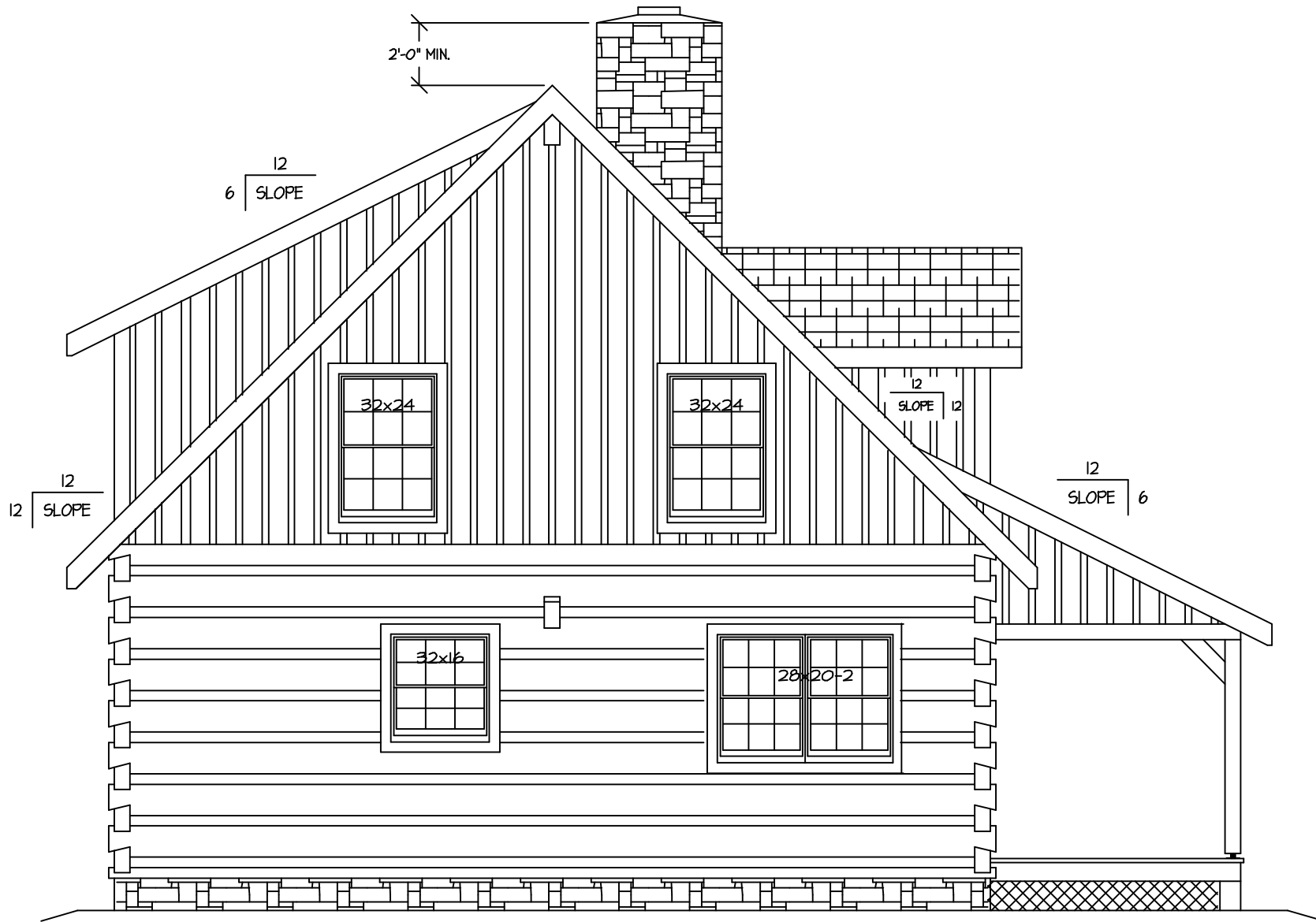
PLAN LEFT ELEVATION
