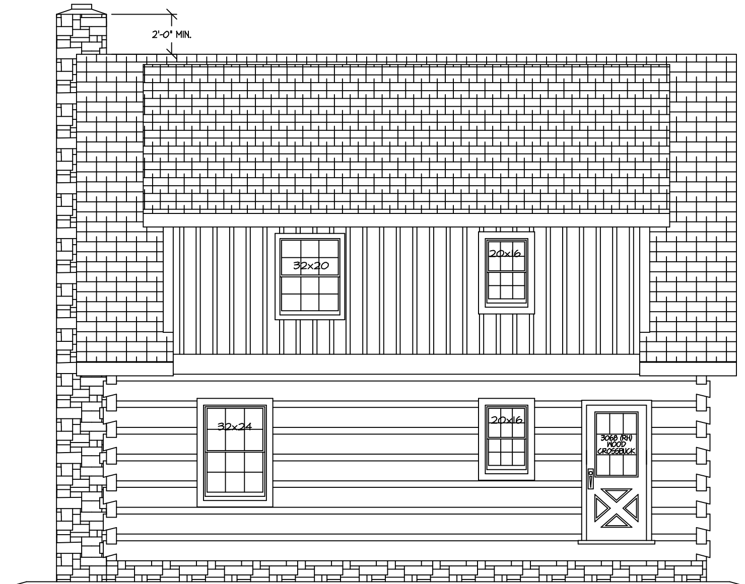
PLAN BACK ELEVATION
