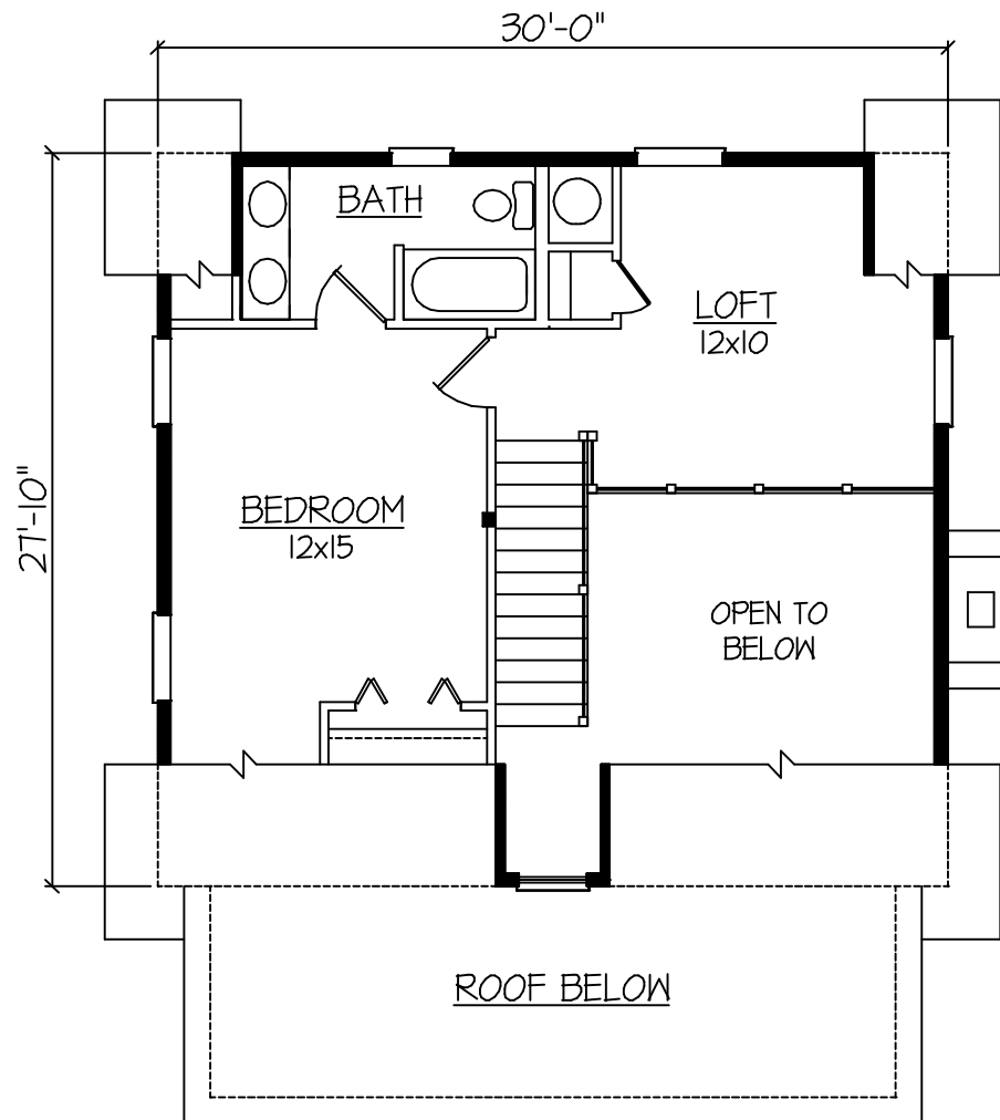
SECOND FLOOR PLAN SECOND FLOOR - 565 SF
