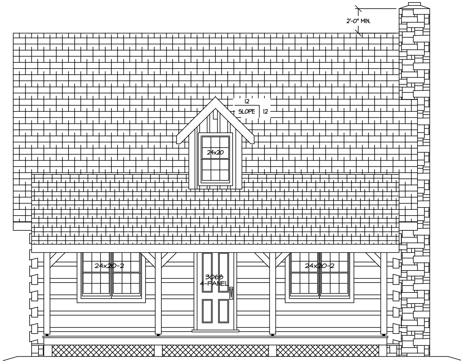
PLAN FRONT ELEVATION
