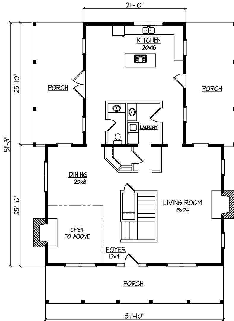
FIRST FLOOR PLAN FIRST FLOOR-15419F TOTAL-2926
