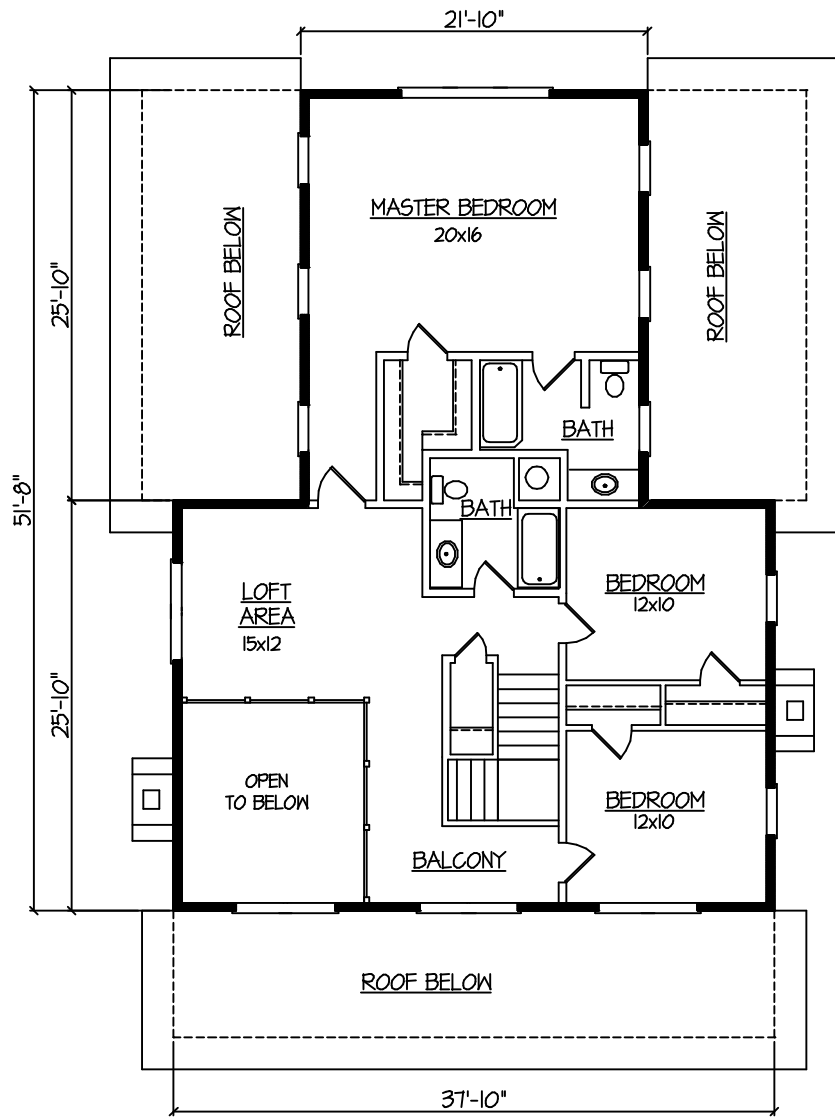
SECOND FLOOR PLAN SECOND FLOOR- 13855F
