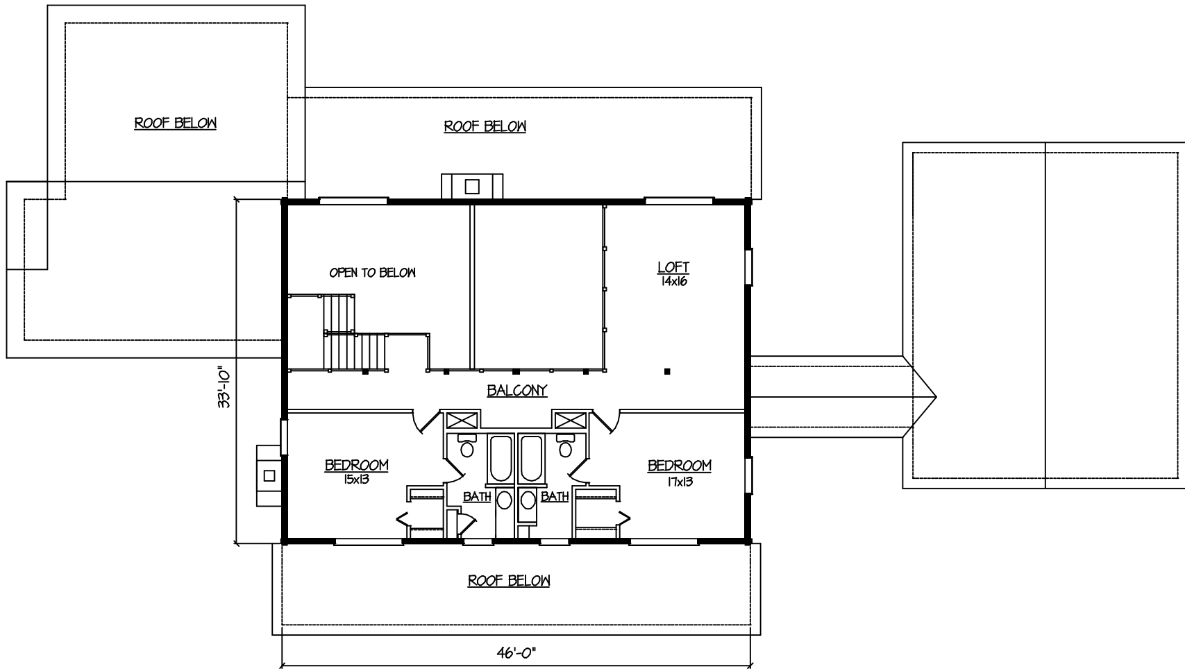
SECOND FLOOR PLAN SECOND FLOOR - 1028 SF
