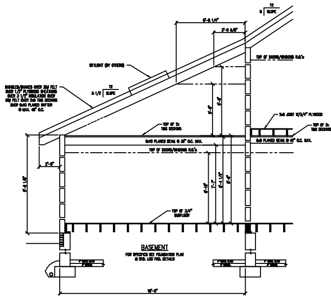
SECTION @ UTILITY/CLOSET
