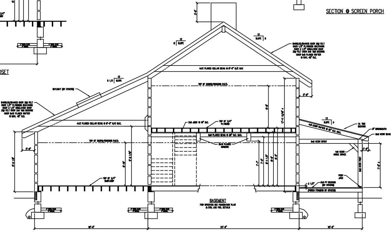
SECTION @ DINING/LIVING/BEDROOMS
