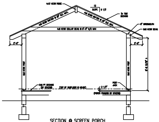
SECTION @ SCREEN PORCH
