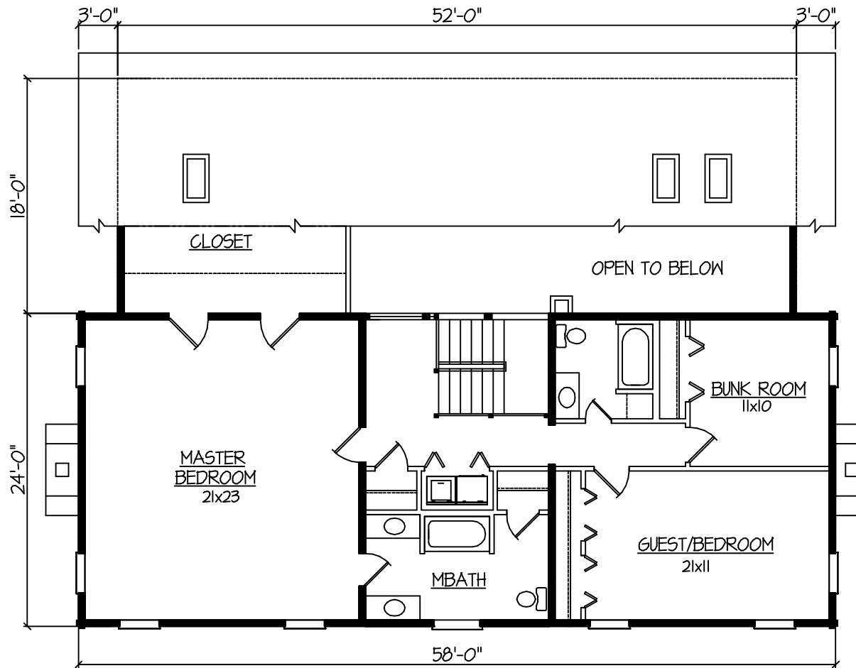
SECOND FLOOR PLAN SECOND FLOOR - 1525 SF
