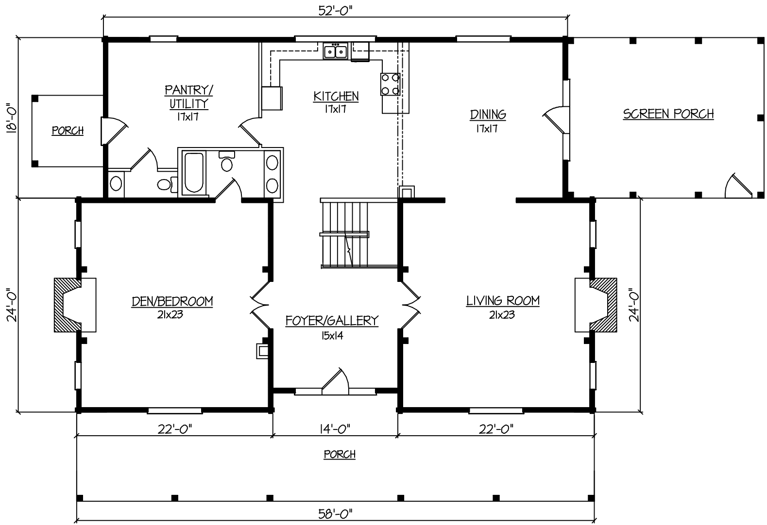
FIRST FLOOR PLAN FIRST FLOOR - 2300SF TOTAL - 3825SF
