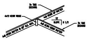
DETAIL @ SCREEN PORCH ROOF
