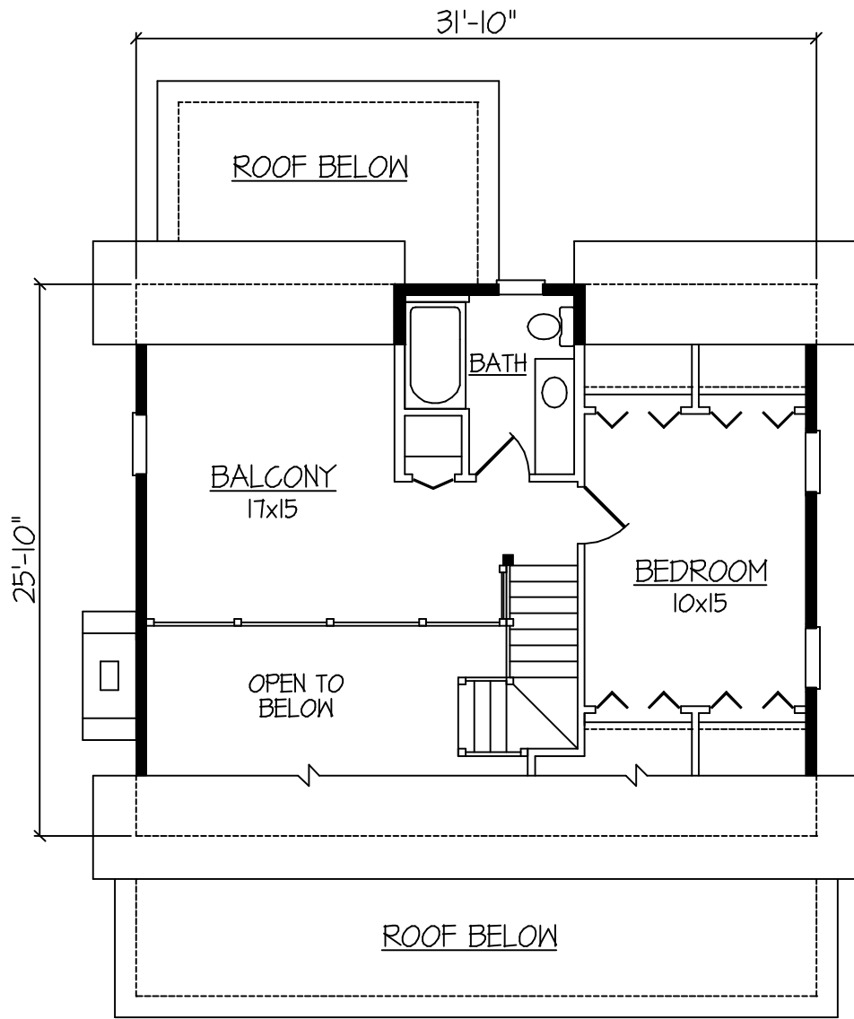
SECOND FLOOR PLAN SECOND FLOOR - 521 SF
