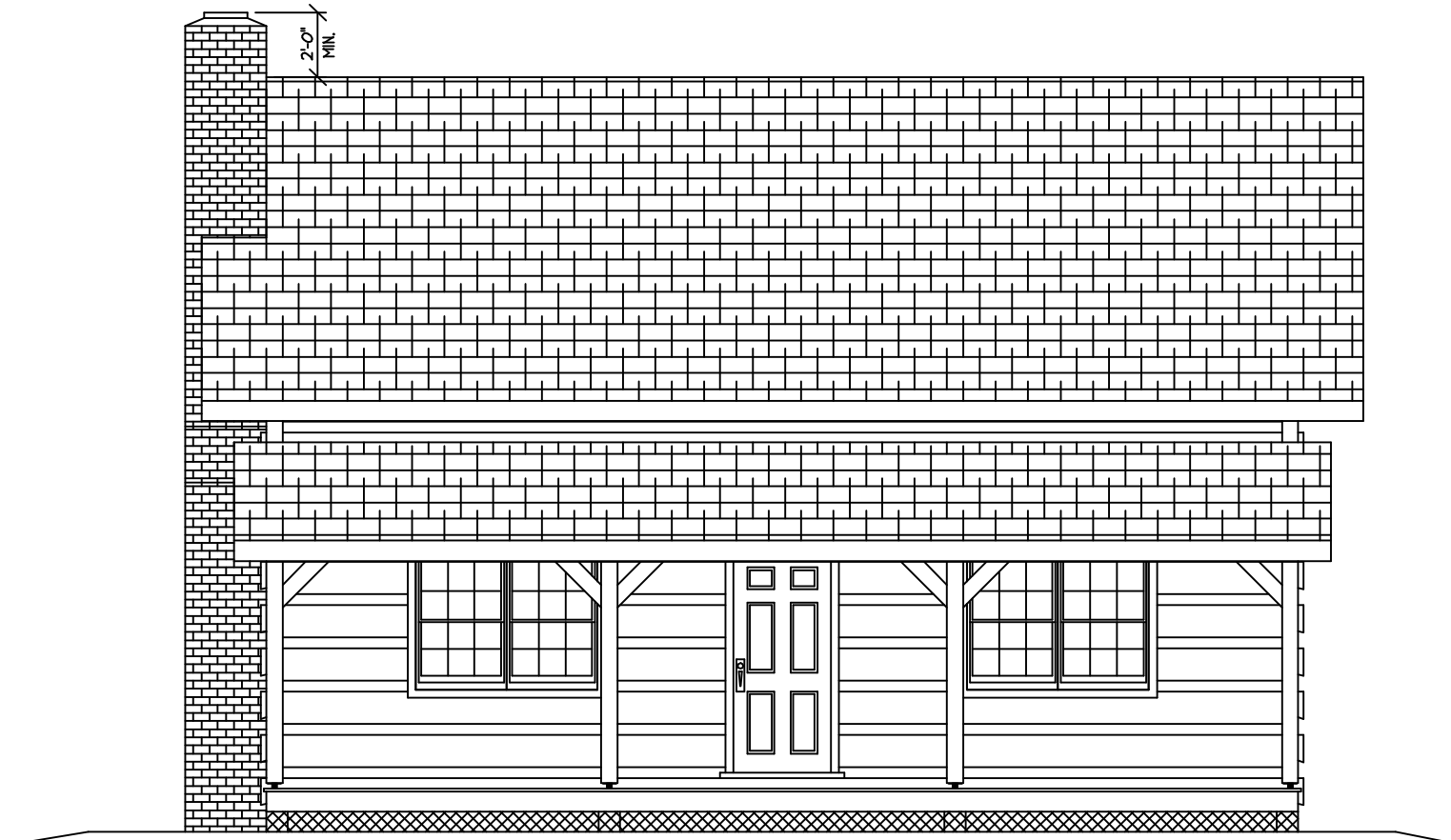
ELEVATION @ FRONT
