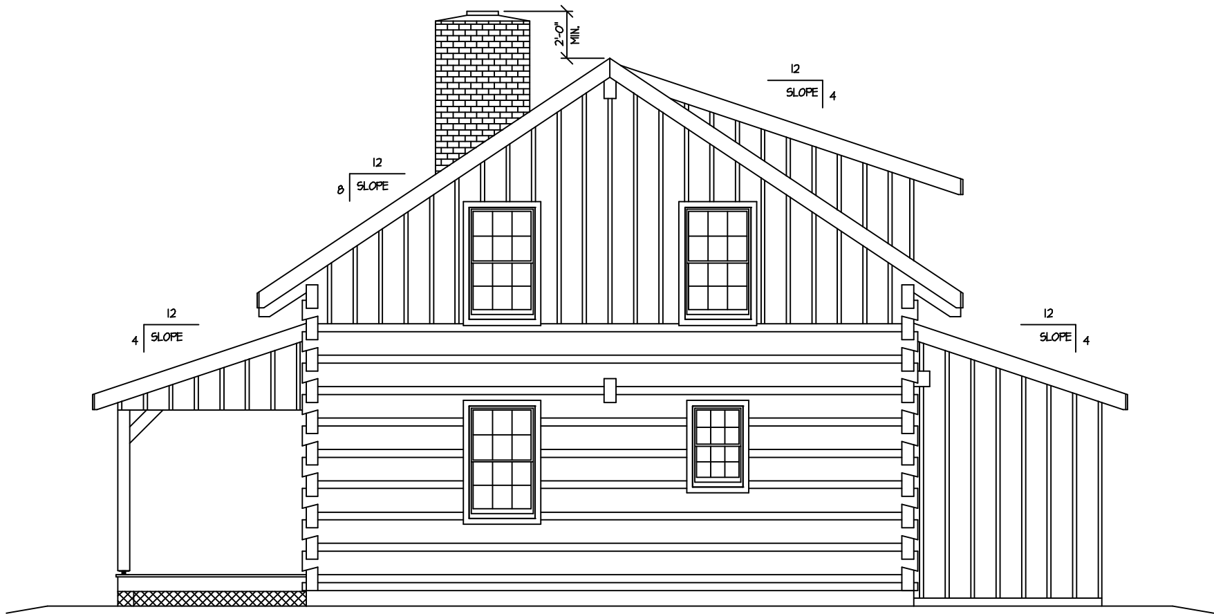
ELEVATION @ RIGHT END
