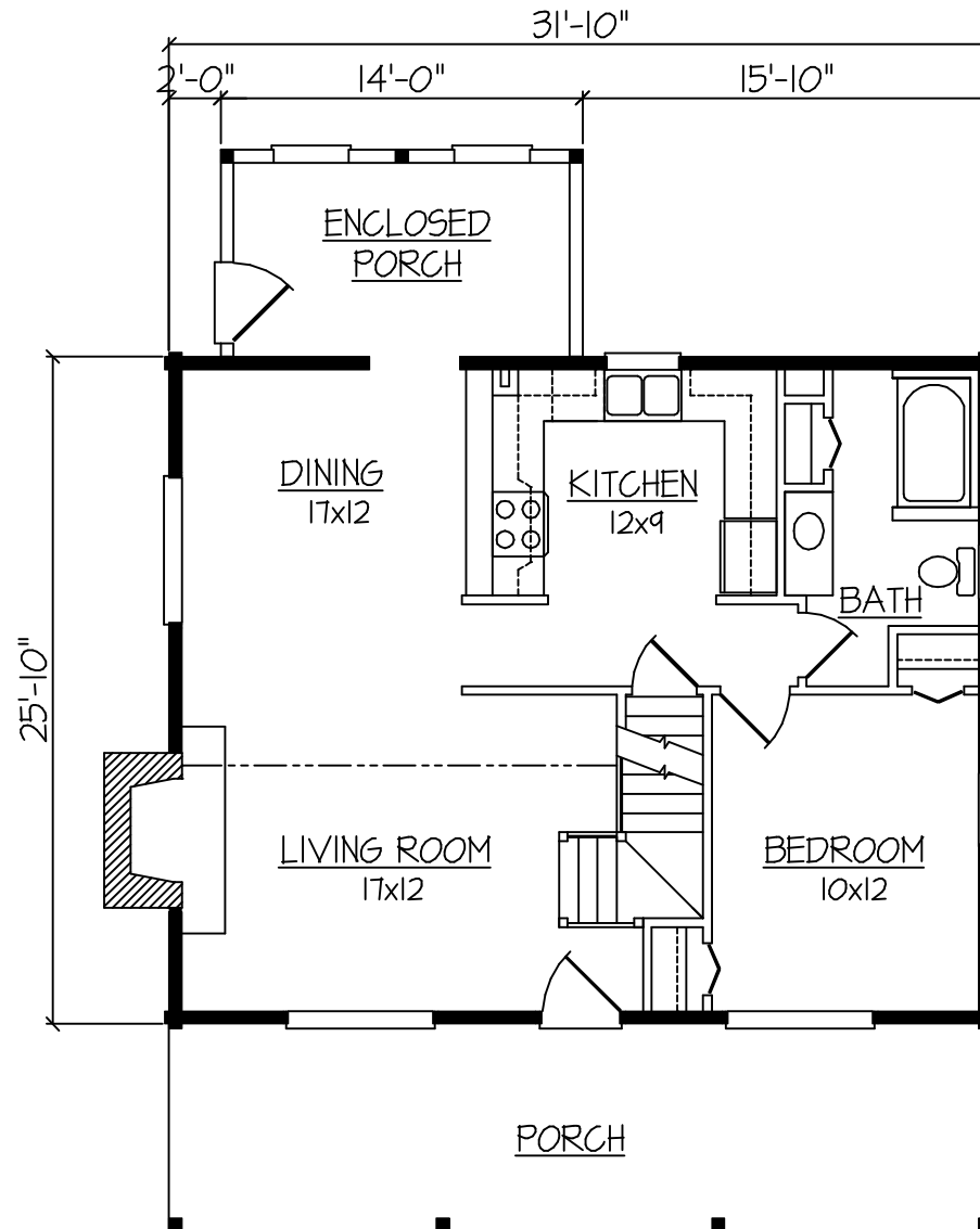
FIRST FLOOR PLAN FIRST FLOOR - 822 SF TOTAL - 1343 SF
