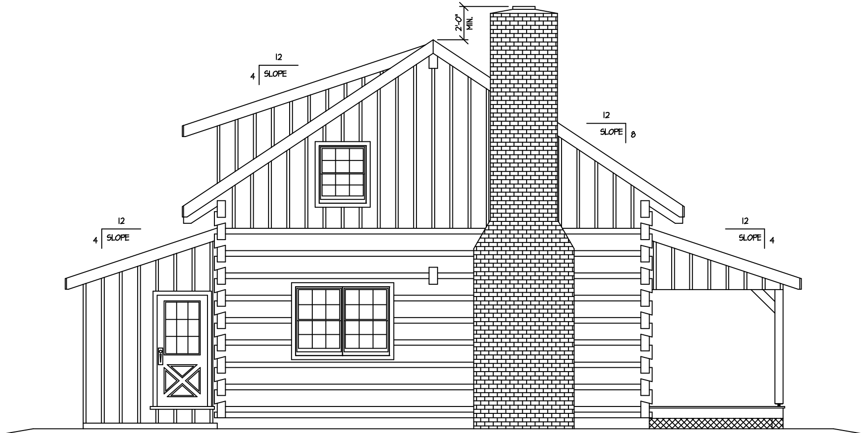
ELEVATION @ LEFT END
