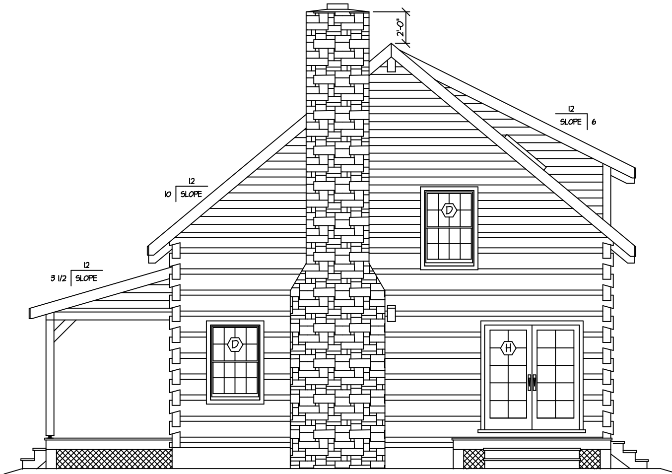
PLAN RIGHT
