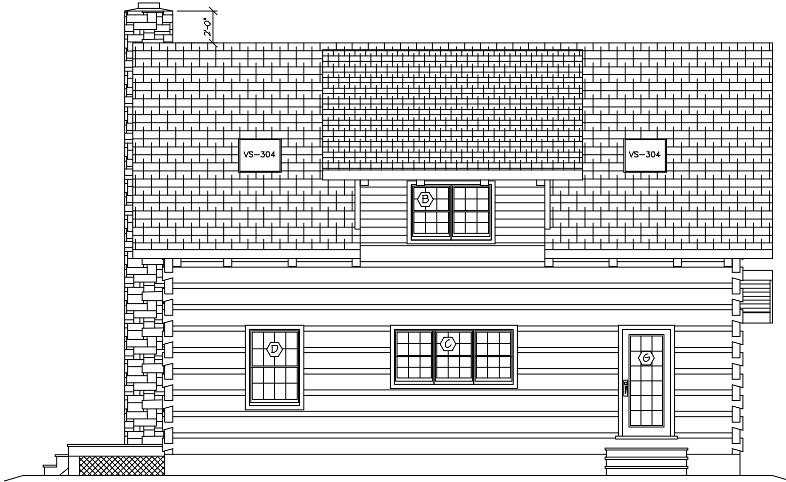
PLAN BACK
