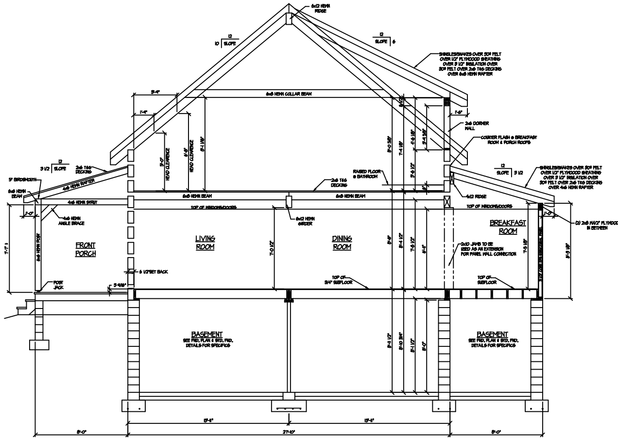
CROSS SECTION @ LIVING/DINING ROOM & BREAKFAST ROOM
