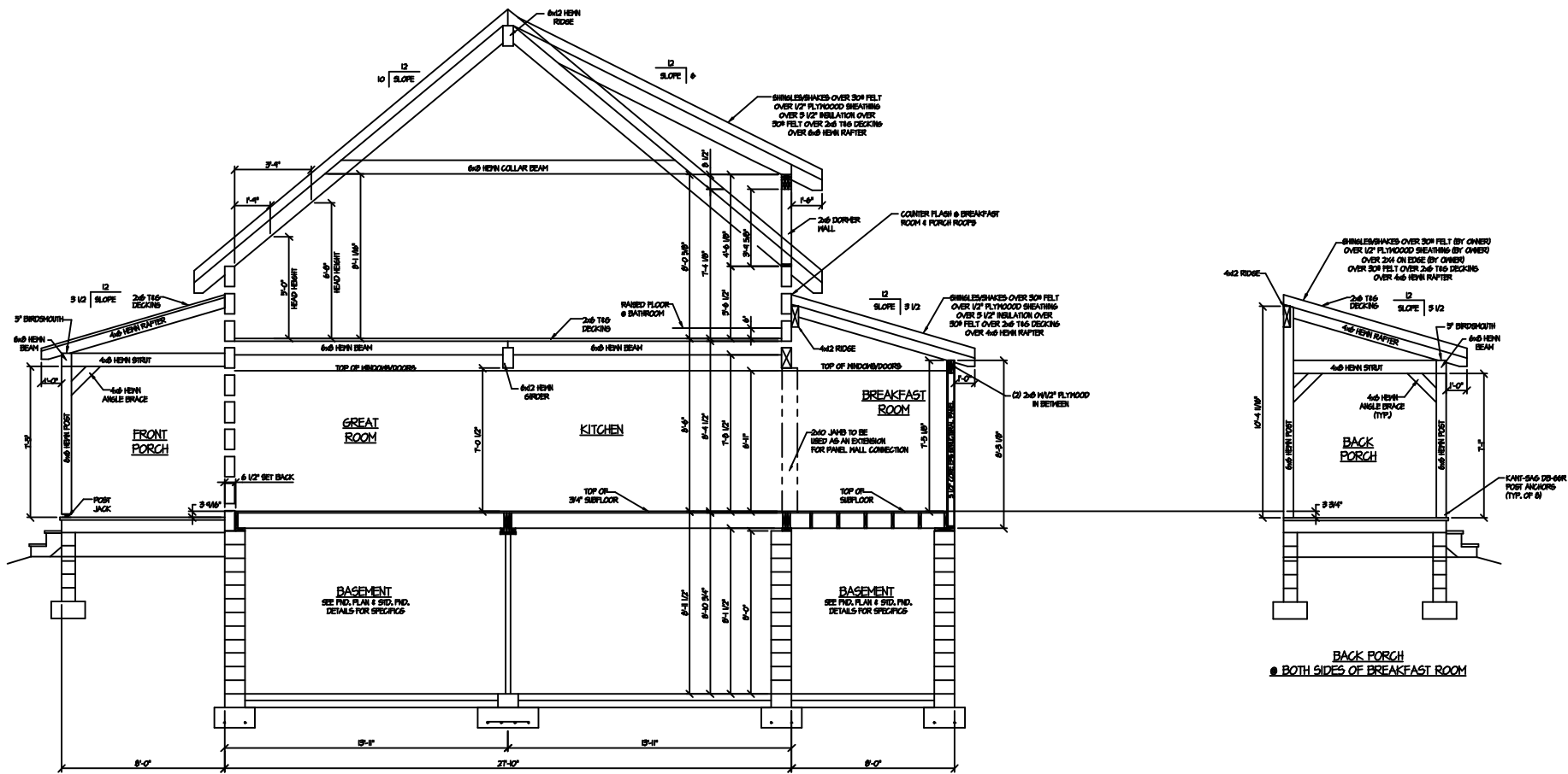
CROSS SECTION @ GREAT ROOM/KITCHEN & BREAKFAST ROOM
