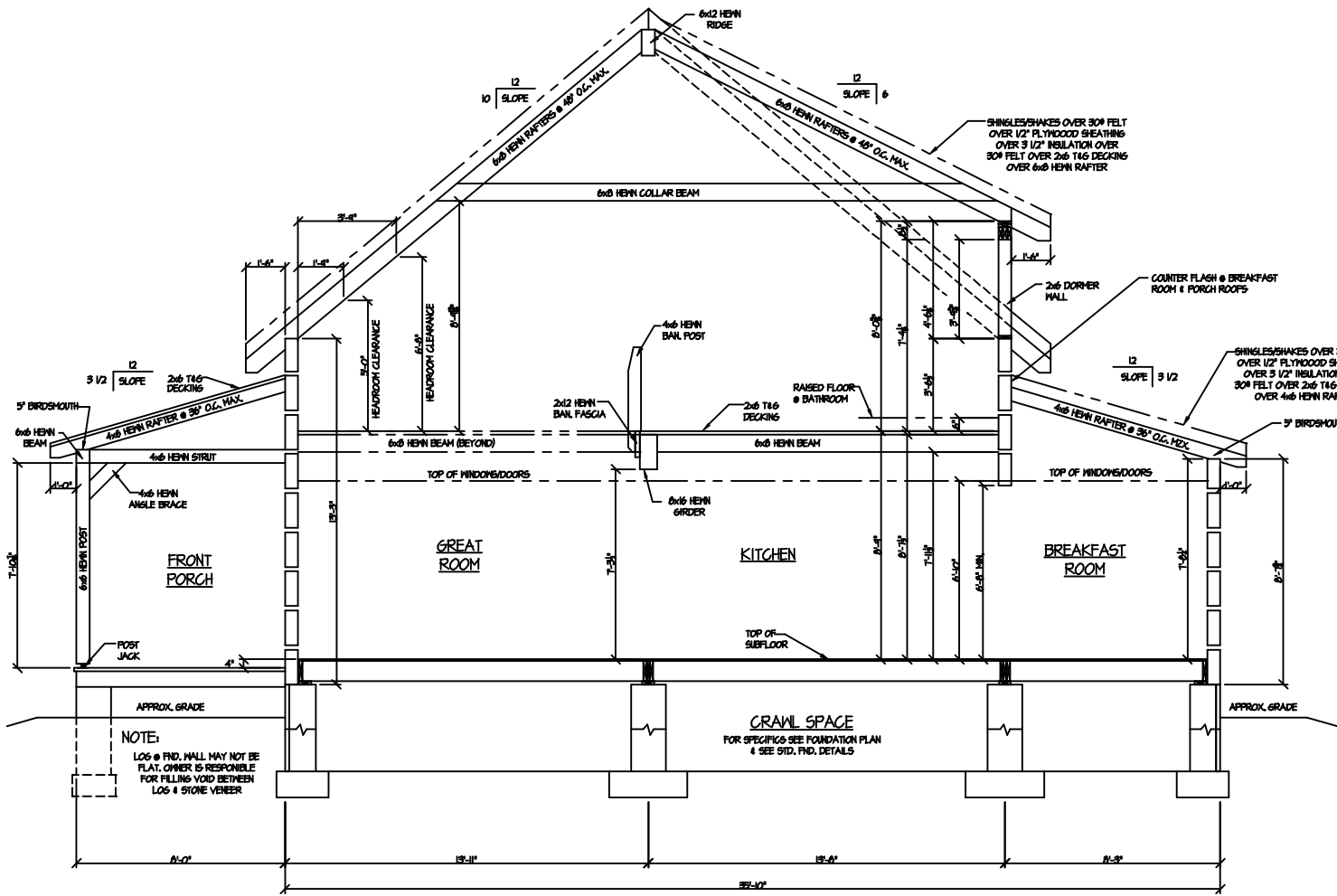
CROSS SECTION @ GREAT ROOM/KITCHEN & BREAKFAST ROOM
