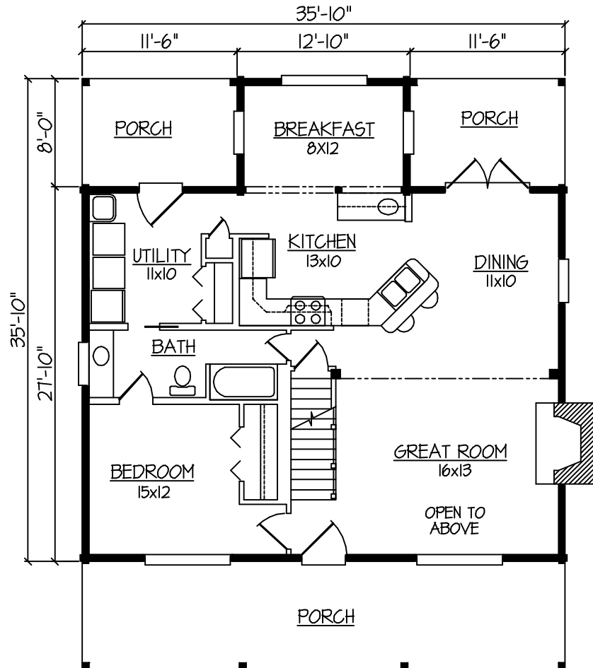
FIRST FLOOR PLAN FIRST FLOOR - 1100 SF TOTAL - 1821 SF
