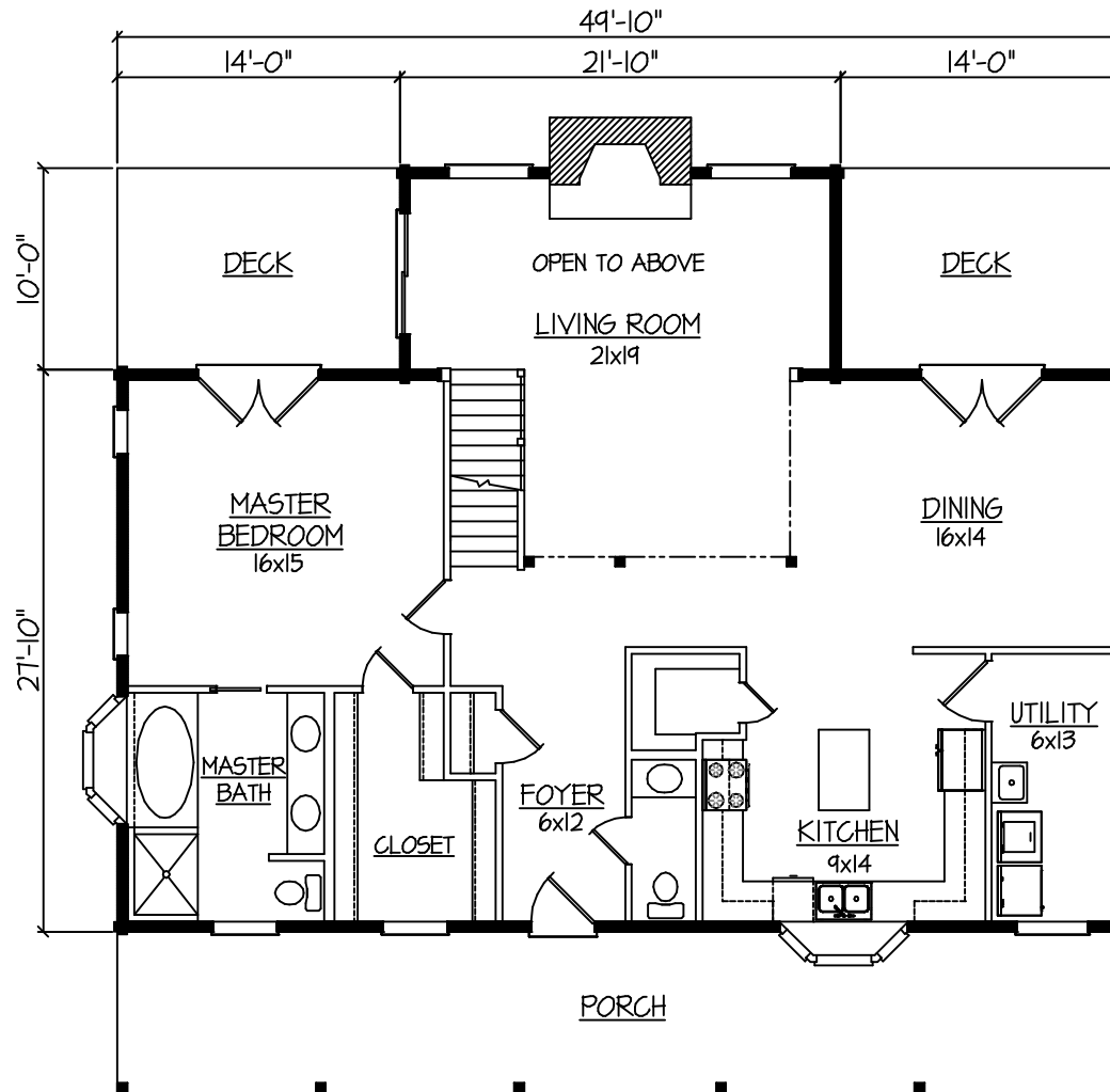
FIRST FLOOR PLAN FIRST FLOOR PLAN - 16055F TOTAL - 25005F
