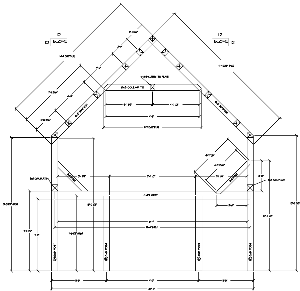
BENTS #1 & #2
