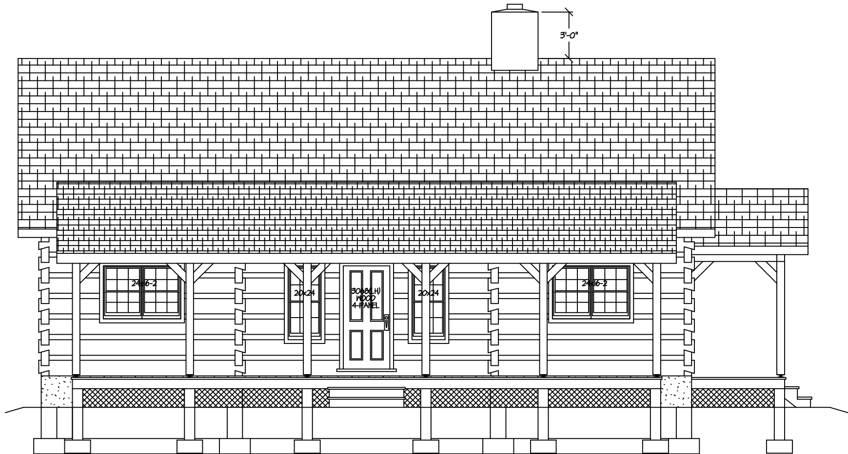
PLAN FRONT
