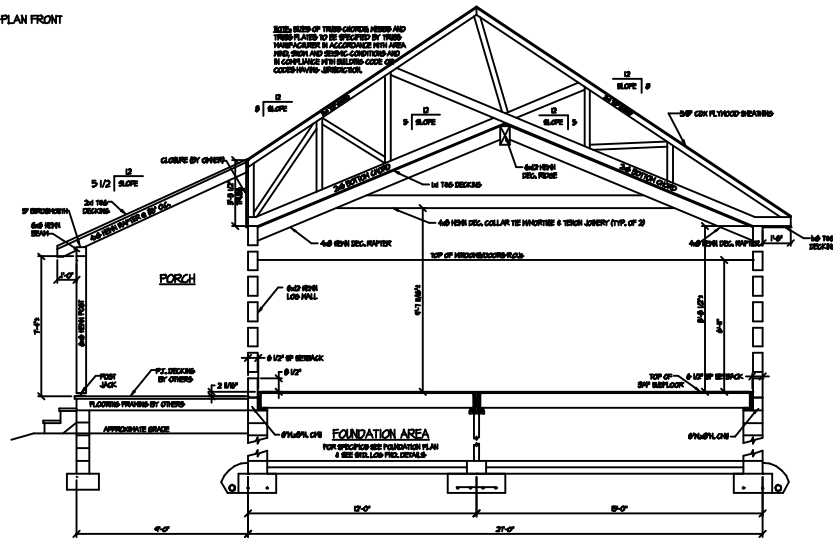
SECTION THRU FOYER/GREAT ROOM/DINING
