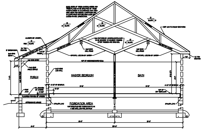
SECTION THRU MASTER BEDROOM/BATH
