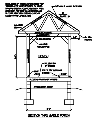
SECTION THRU GABLE PORCH
