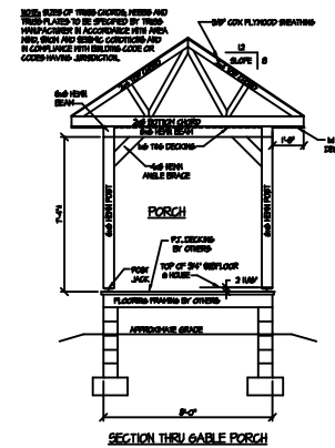
SECTION THRU GABLE PORCH
