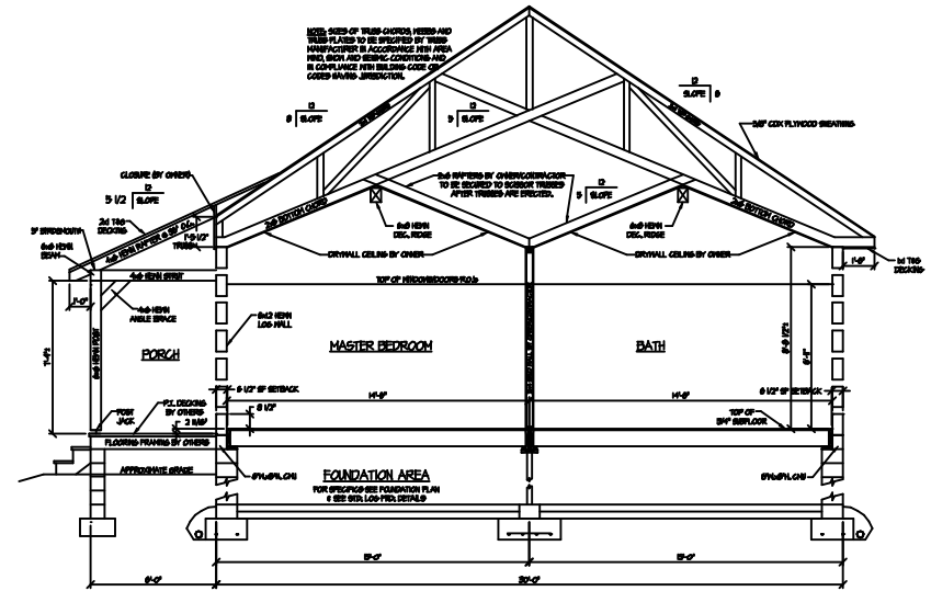
SECTION THRU MASTER BEDROOM/BATH/KITCHEN
