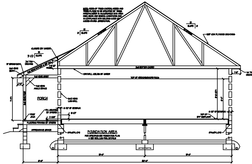
SECTION THRU BEDROOM/BATH/BEDROOM
