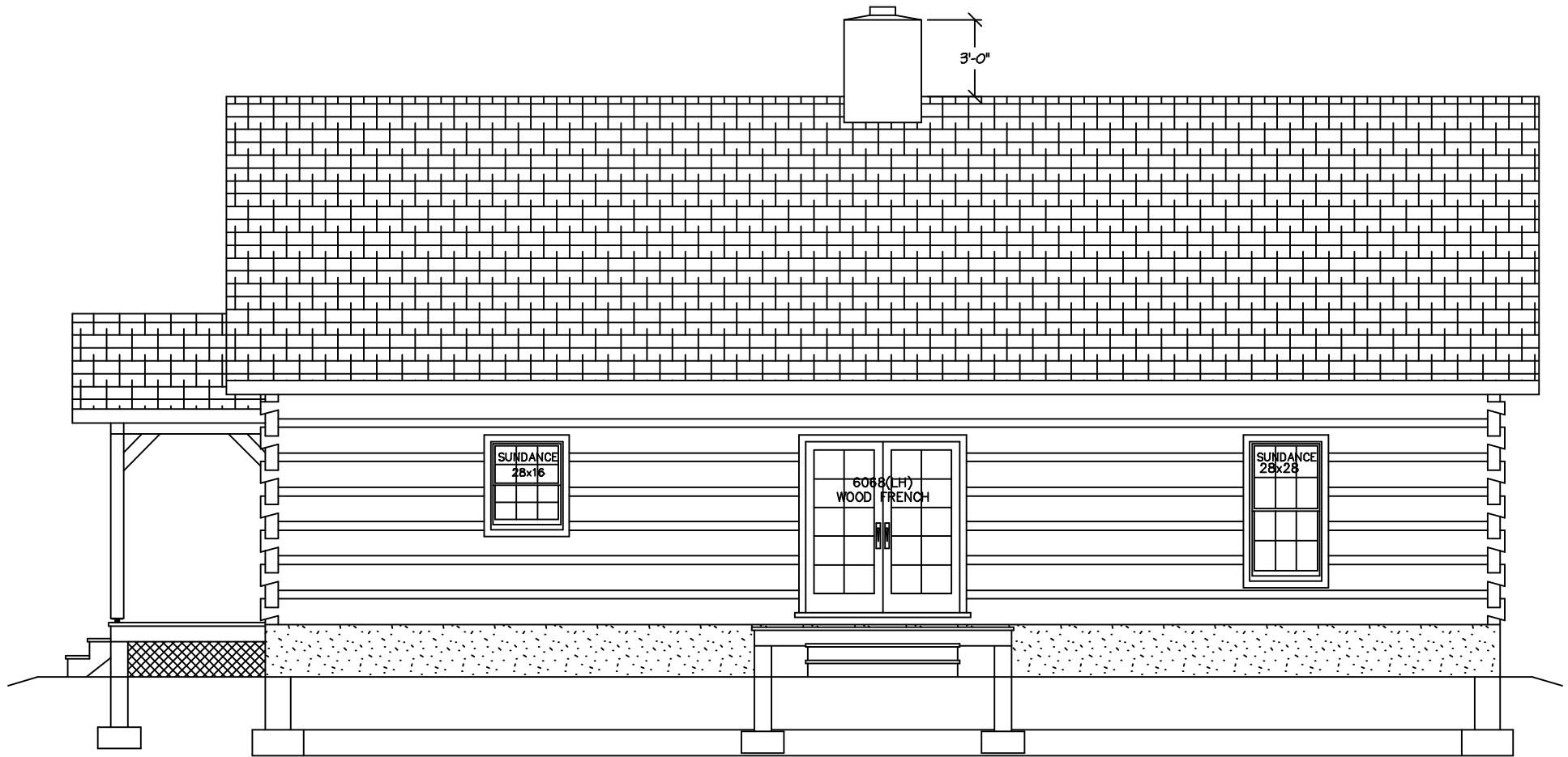
PLAN BACK
