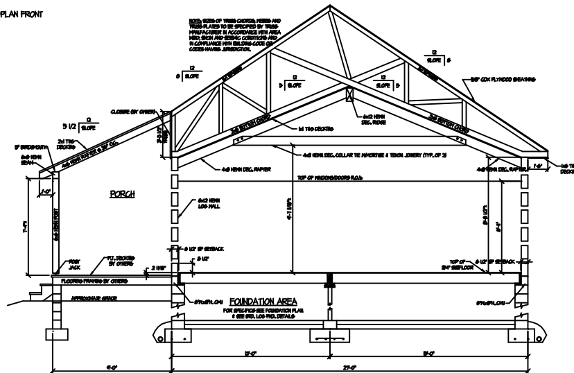
SECTION THRU GREAT ROOM/DINING
