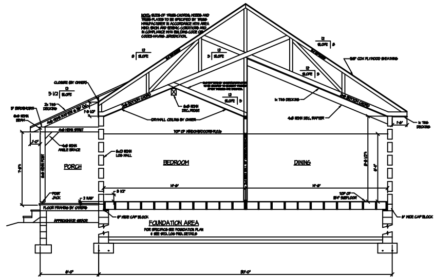
SECTION THRU BEDROOM/DINING
