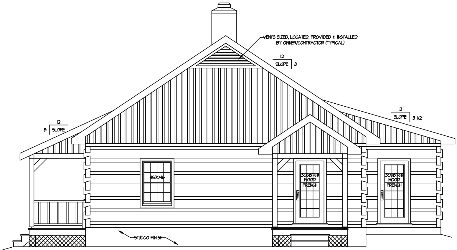
PLAN RIGHT
