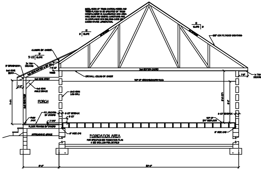
SECTION THRU BEDROOM/BATH
