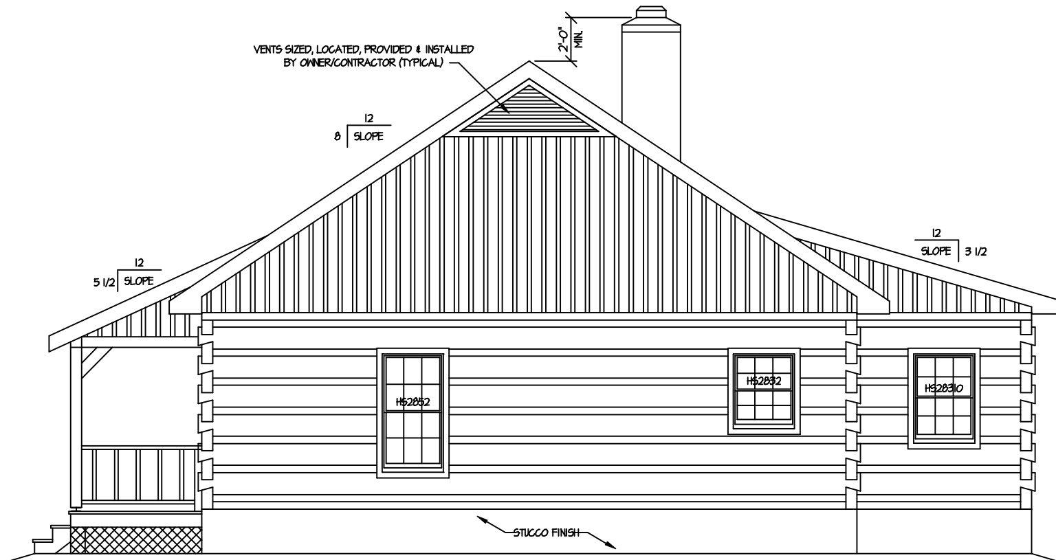
PLAN RIGHT
