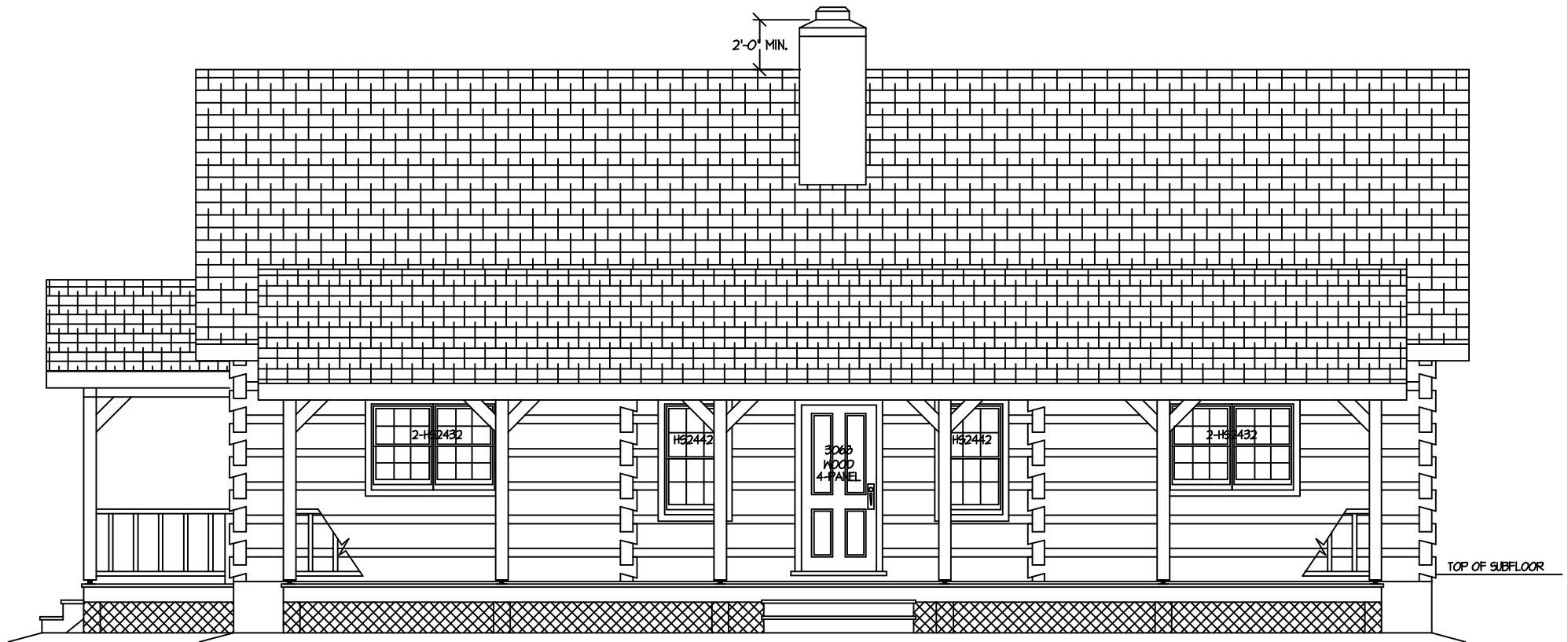
PLAN FRONT
