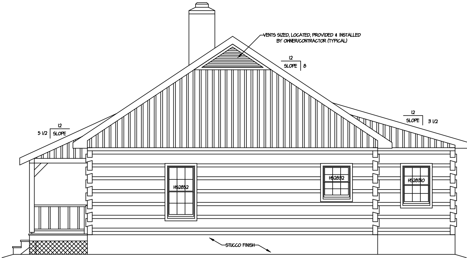
PLAN RIGHT
