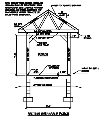
SECTION THRU GABLE PORCH
