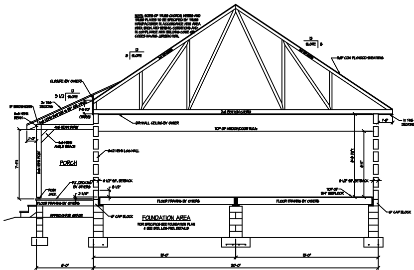
SECTION THRU BEDROOM/BATH/REARDOOR
