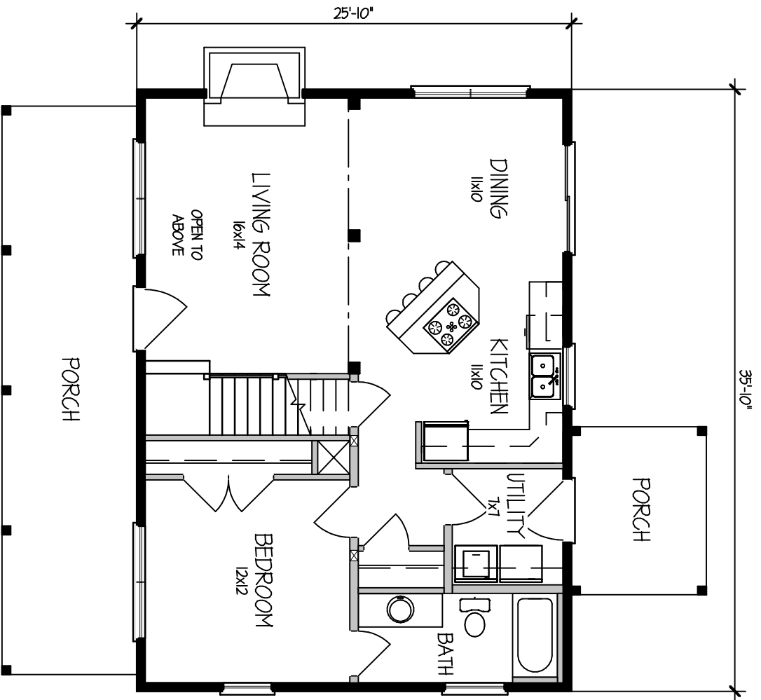
FIRST FLOOR PLAN FIRST FLOOR PLAN - 925 SF TOTAL - 1536 SF
