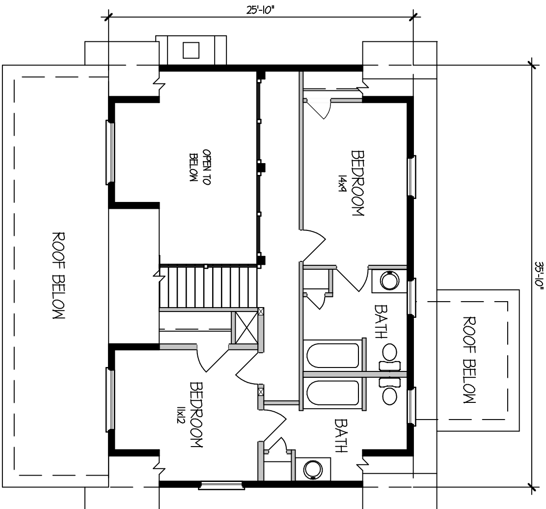
SECOND FLOOR PLAN SECOND FLOOR PLAN - 611 SF
