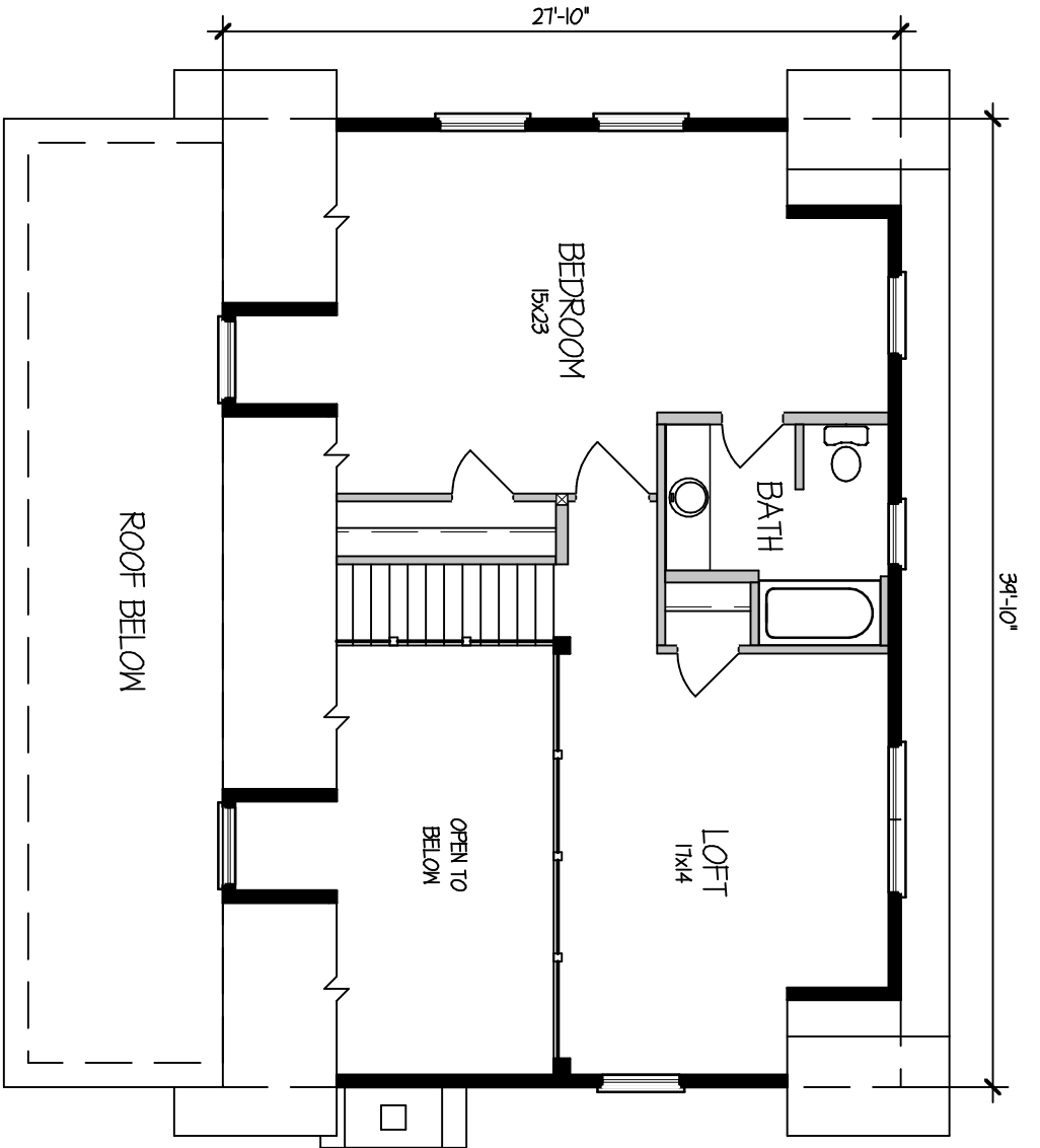
SECOND FLOOR PLAN SECOND FLOOR PLAN - 668 SF
