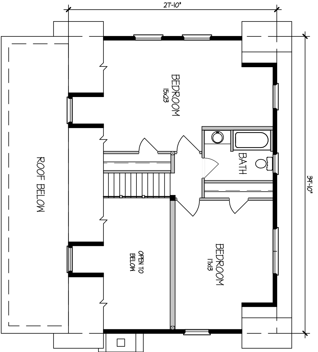
SECOND FLOOR PLAN SECOND FLOOR PLAN - 668 SF
