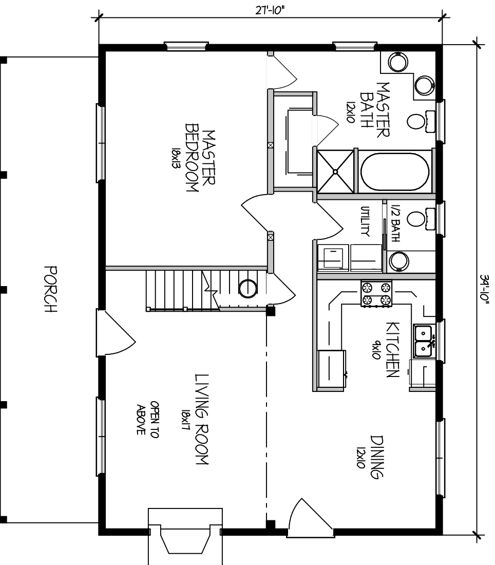
FIRST FLOOR PLAN FIRST FLOOR PLAN - 1108 SF TOTAL - 1776 SF
