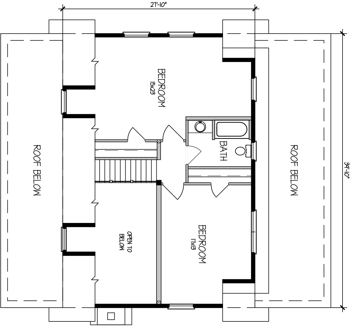
SECOND FLOOR PLAN SECOND FLOOR PLAN - 668 SF
