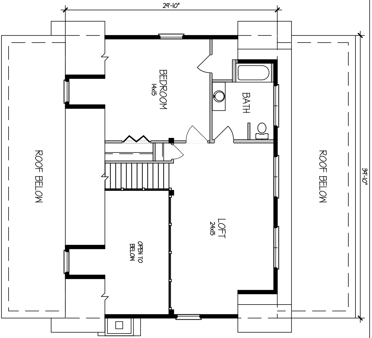
SECOND FLOOR PLAN SECOND FLOOR PLAN - 748 SF
