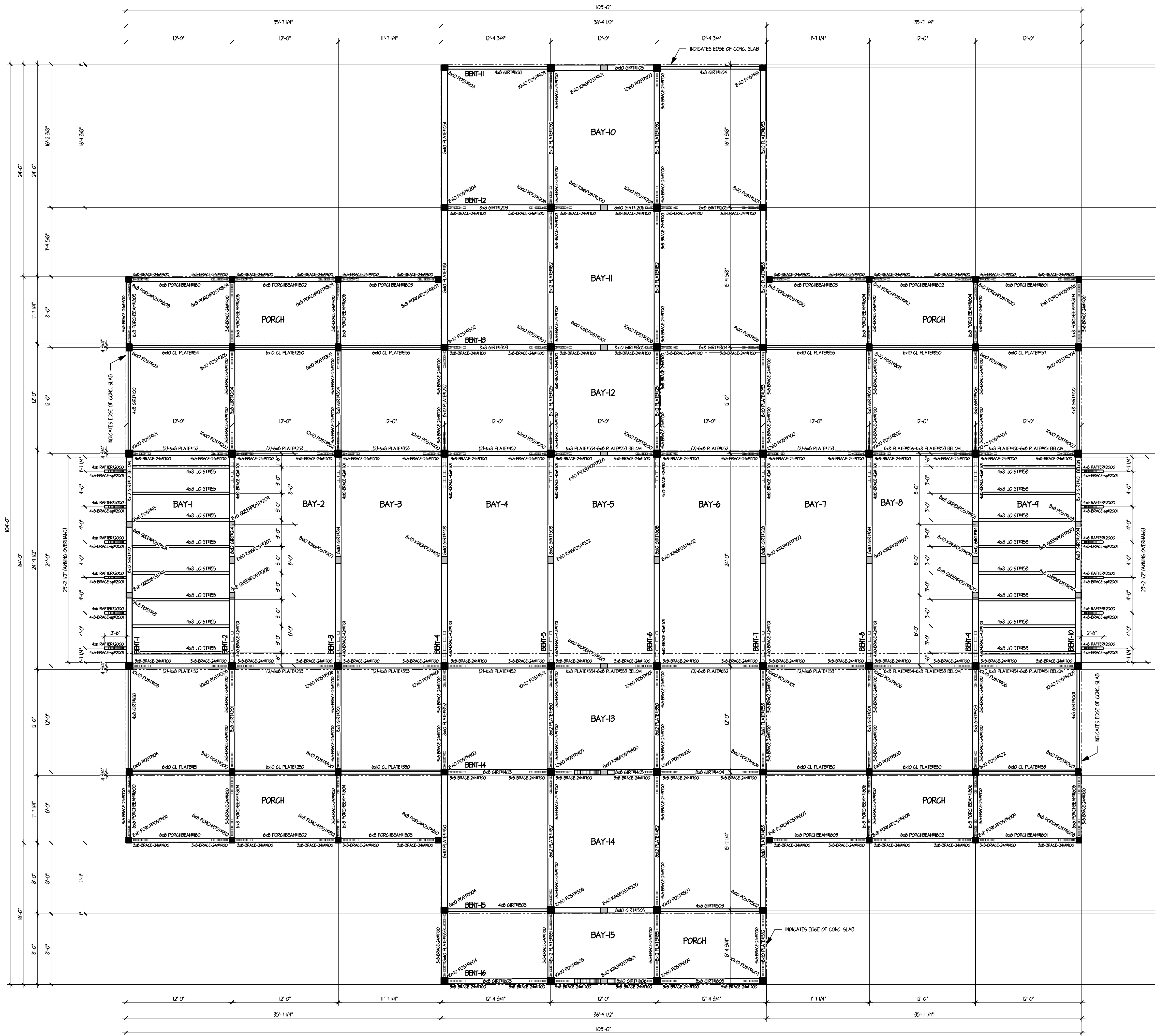
PLAN FRONT POST/LOFT FRAMING PLAN
