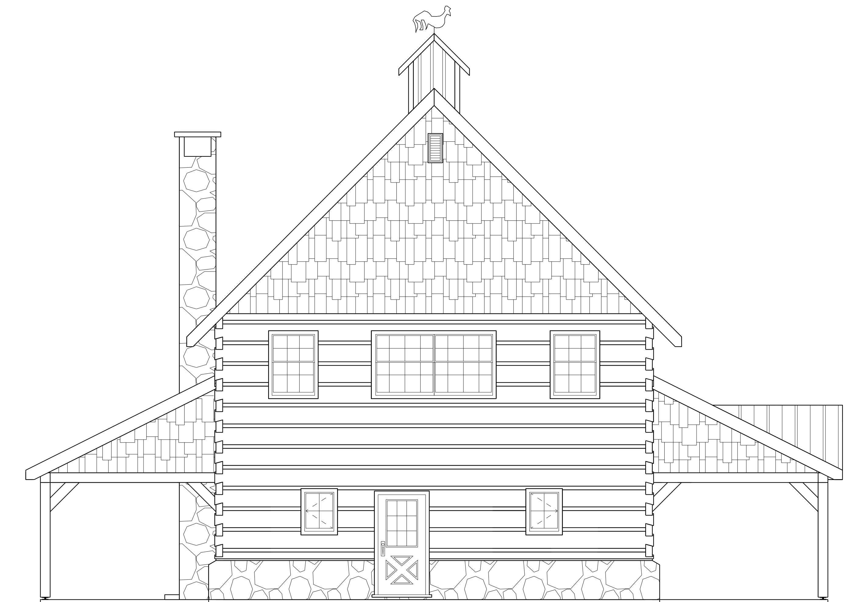
PLAN RIGHT ELEVATION
