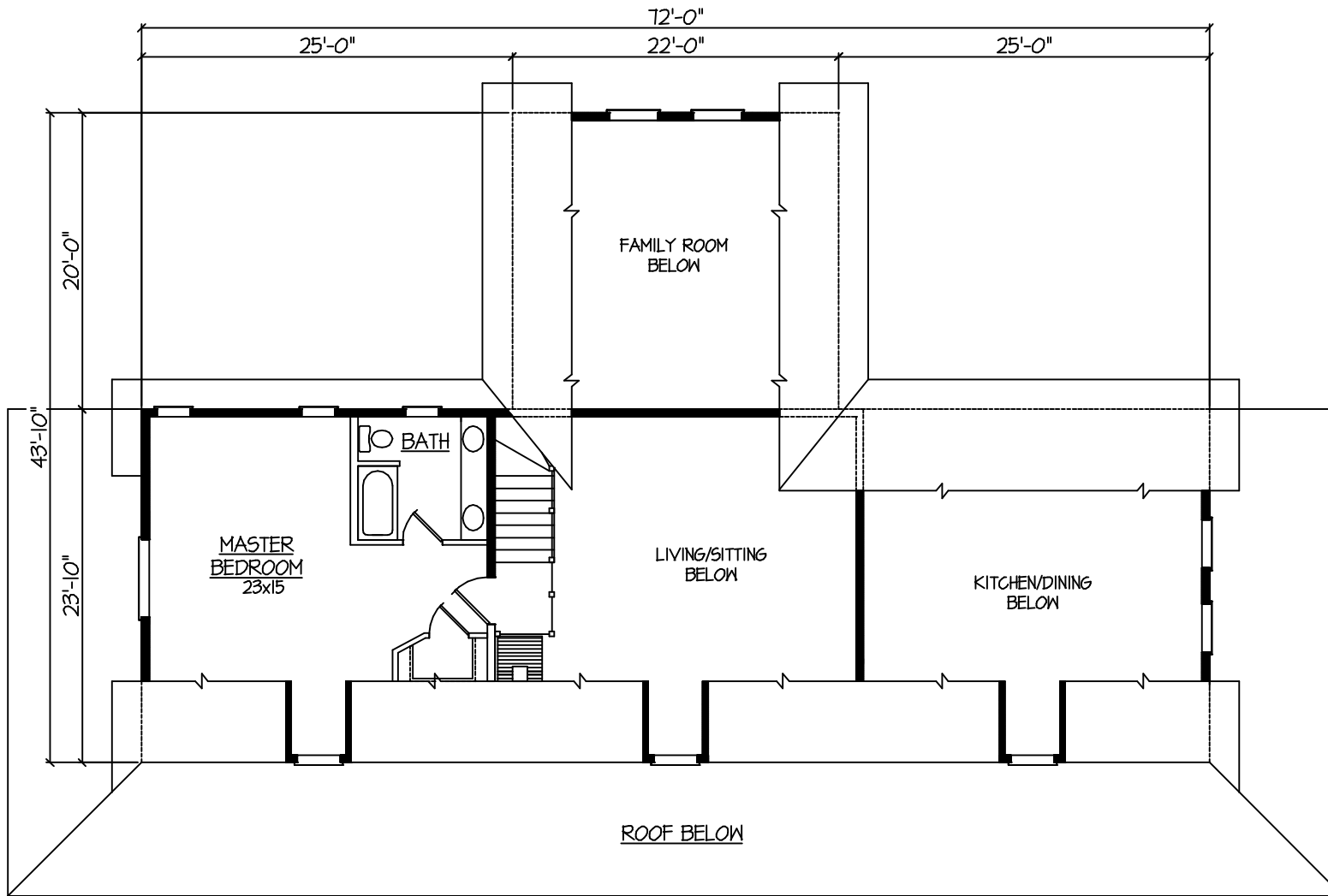
SECOND FLOOR PLAN SECOND FLOOR - 428 SF
