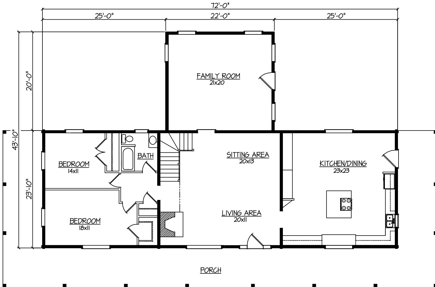
FIRST FLOOR PLAN FIRST FLOOR - 2155 SF TOTAL - 2583 SF
