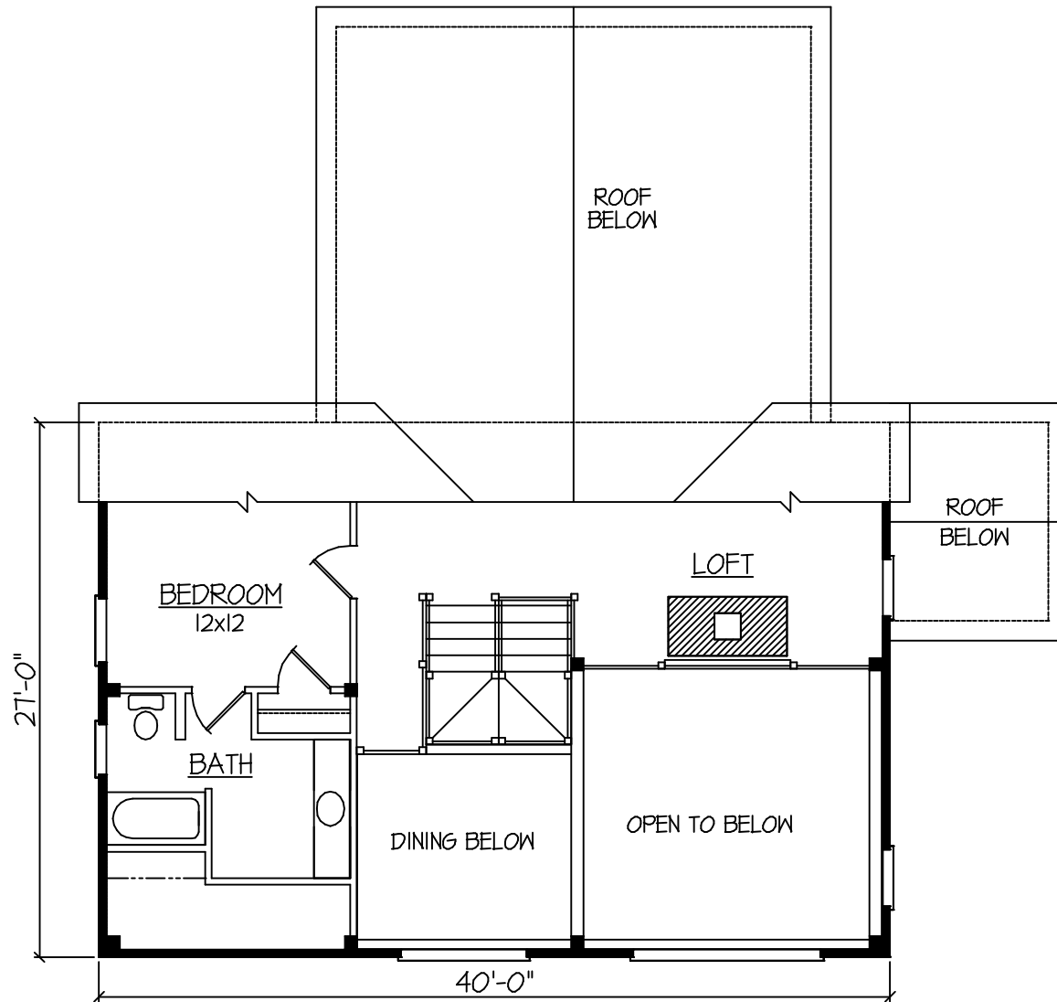
SECOND FLOOR PLAN SECOND FLOOR - 536 SF
