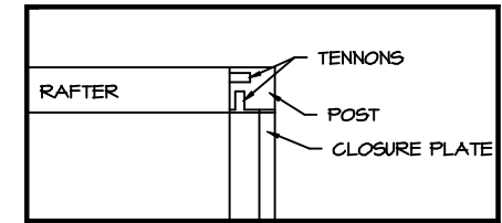
POST & RAFTER DETAIL SCALE: 1" = 1'-0"
