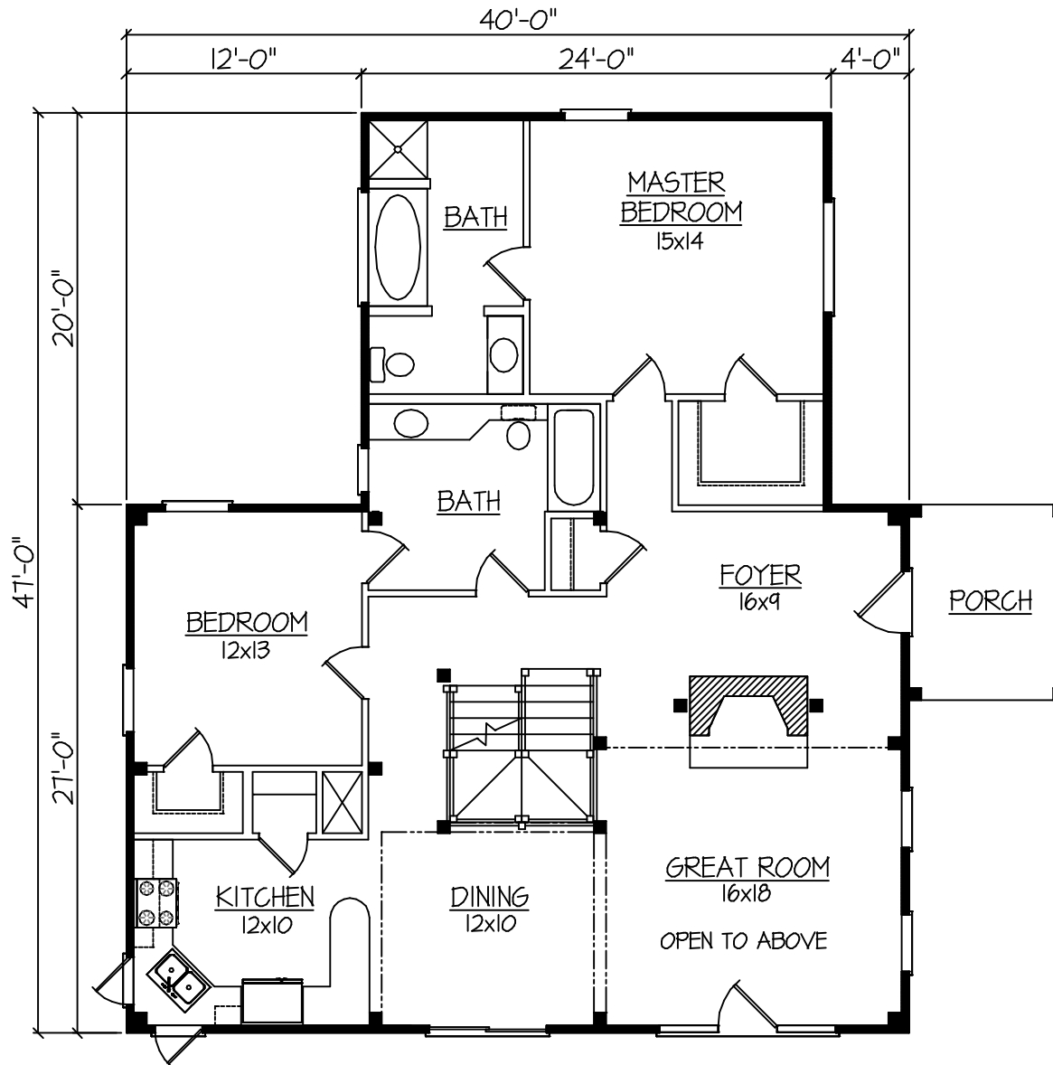
FIRST FLOOR PLAN FIRST FLOOR - 1560 SF TOTAL - 2096 SF
