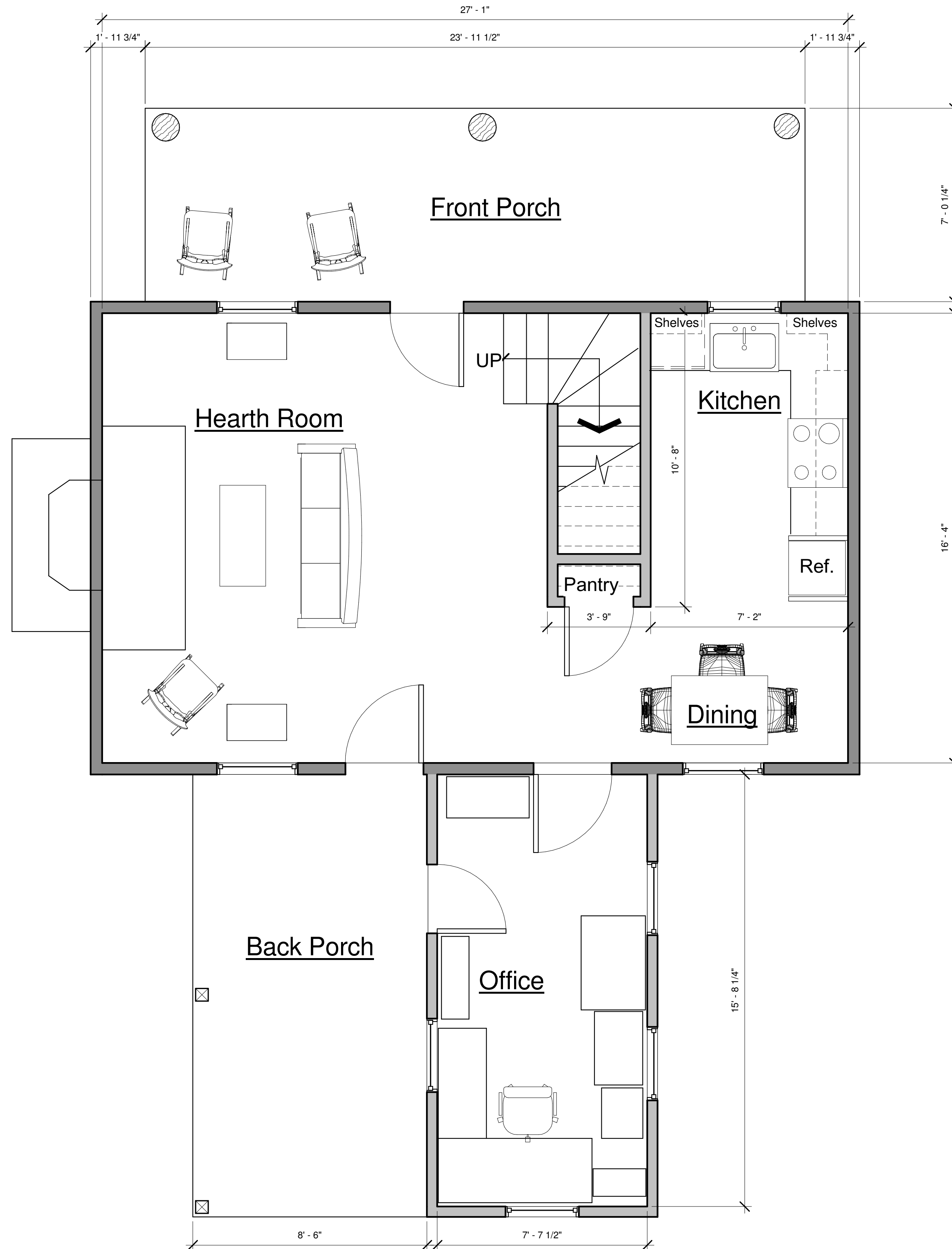
① First Floor 3/8" = 1'-0"
