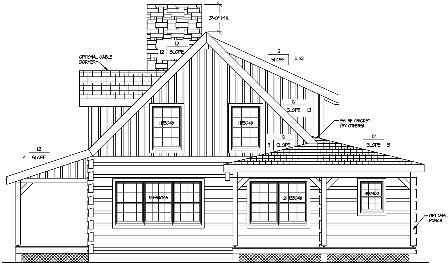
PLAN RIGHT
