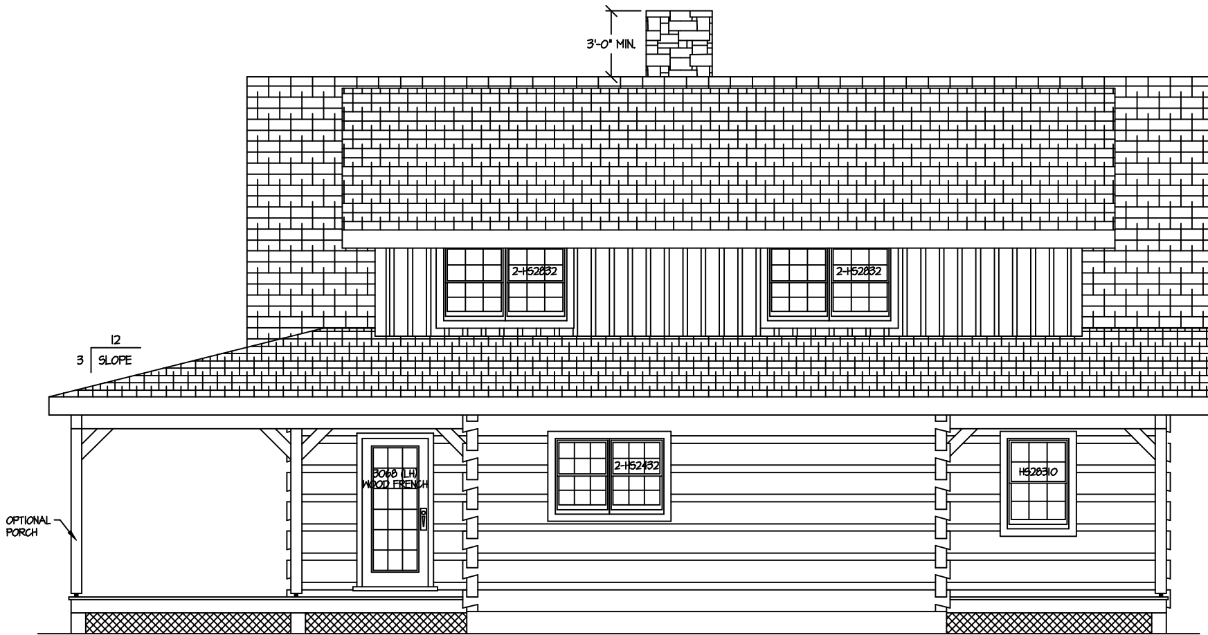
PLAN REAR
