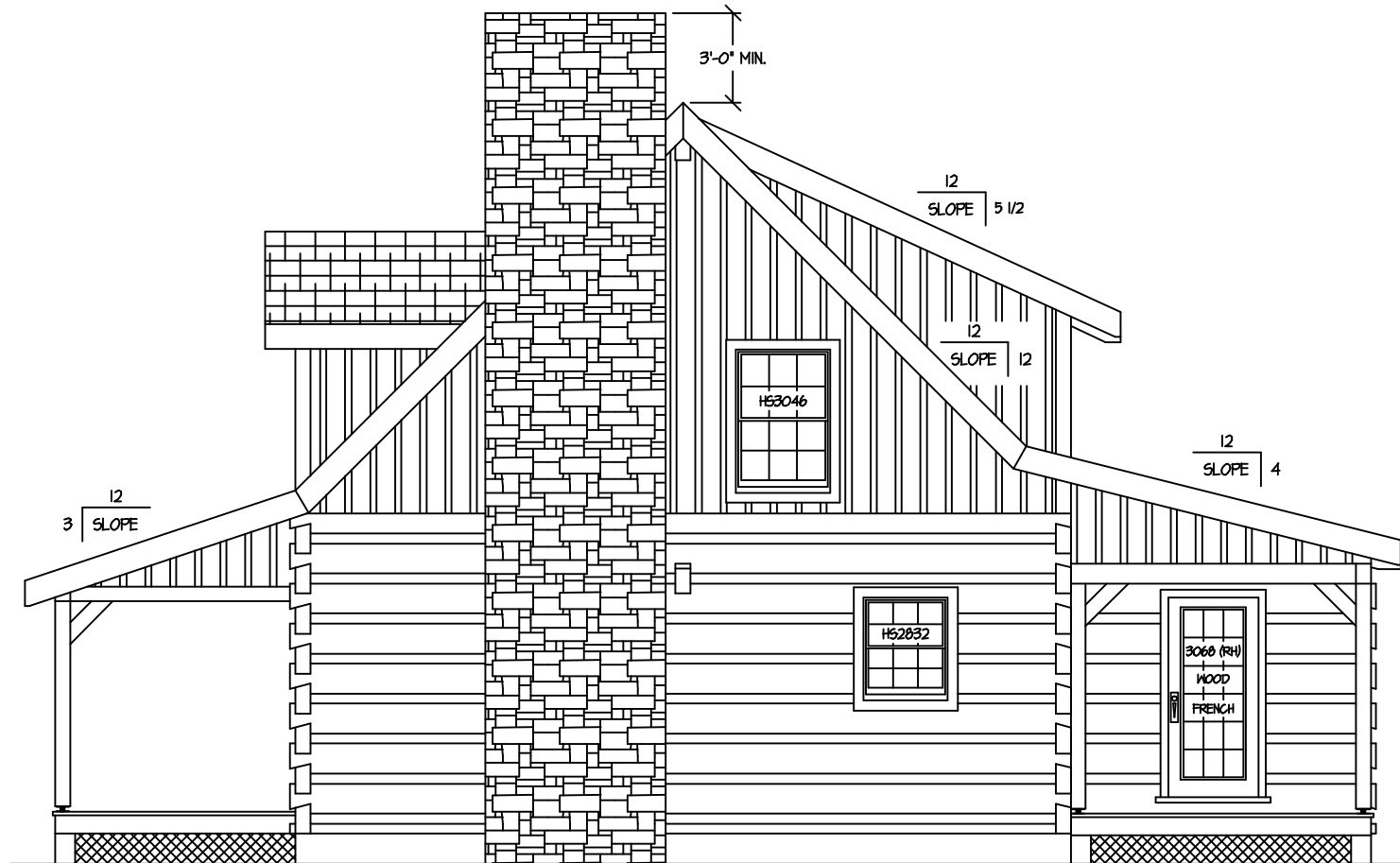
PLAN RIGHT
