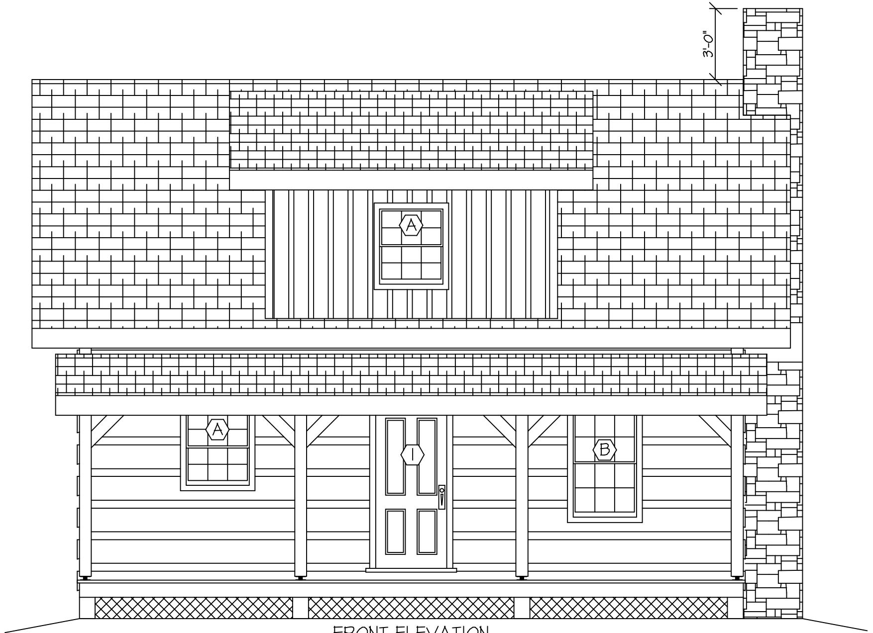
FRONT ELEVATION
