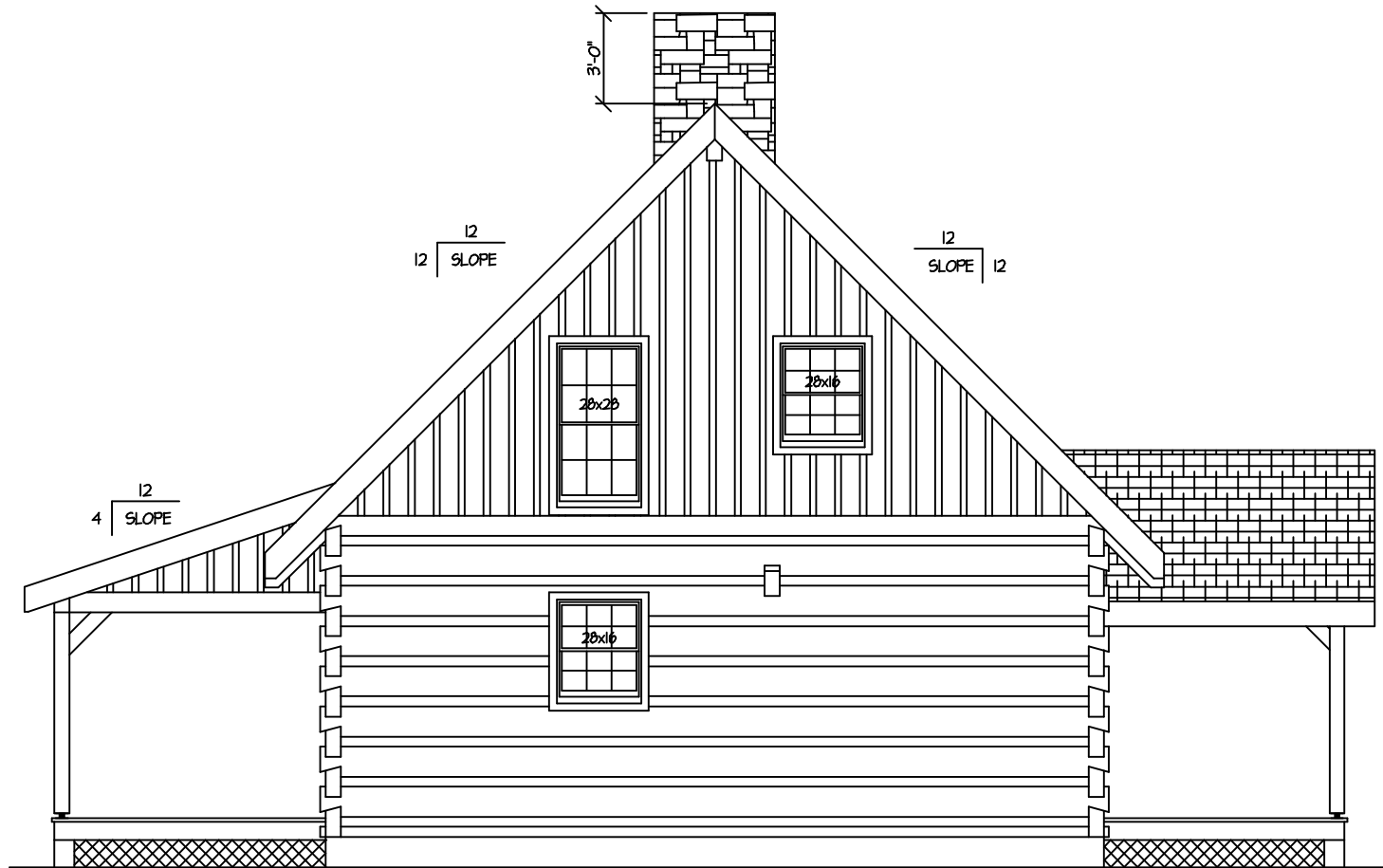
PLAN RIGHT
