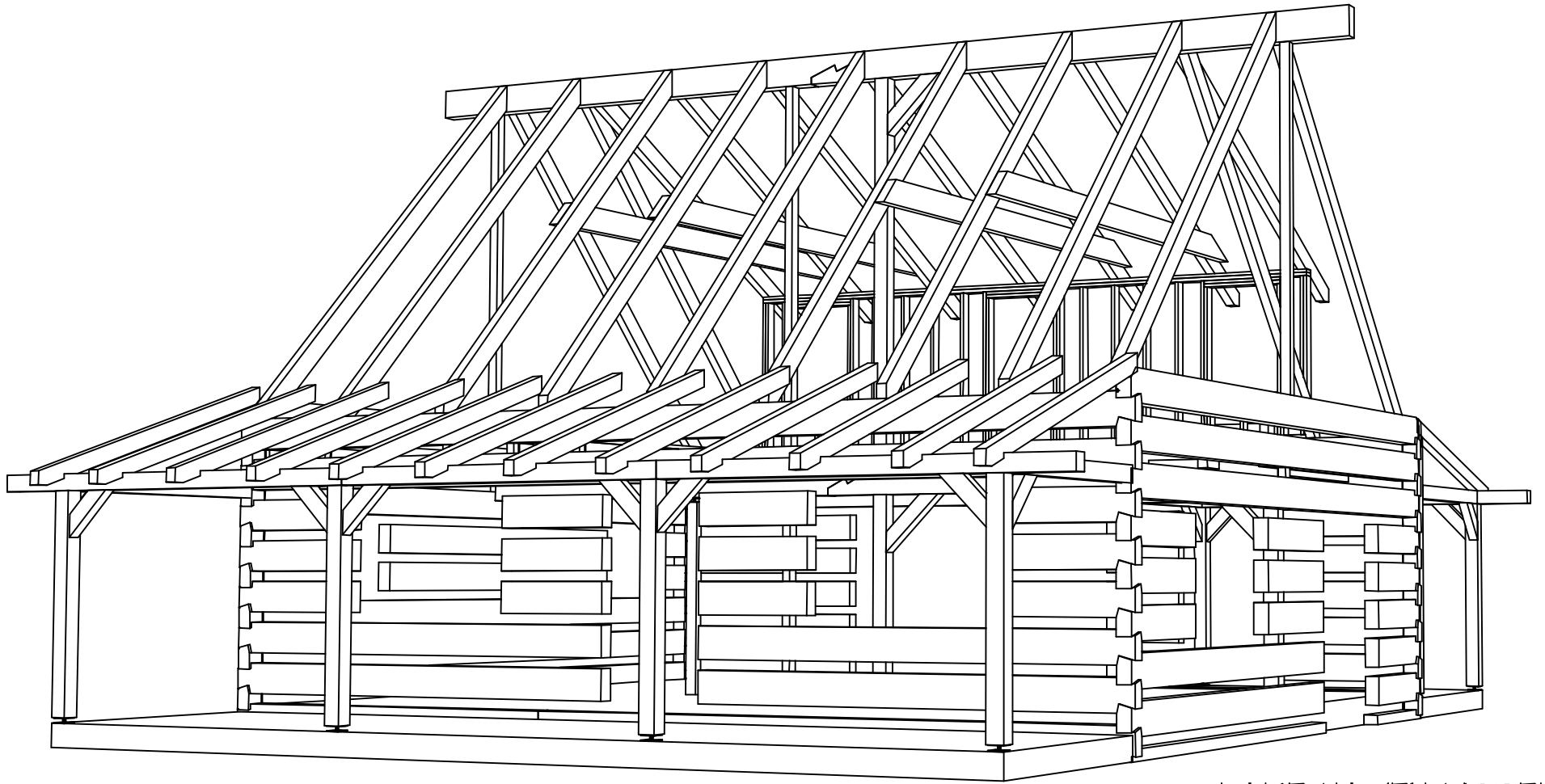
LAKE HAVEN MODEL
