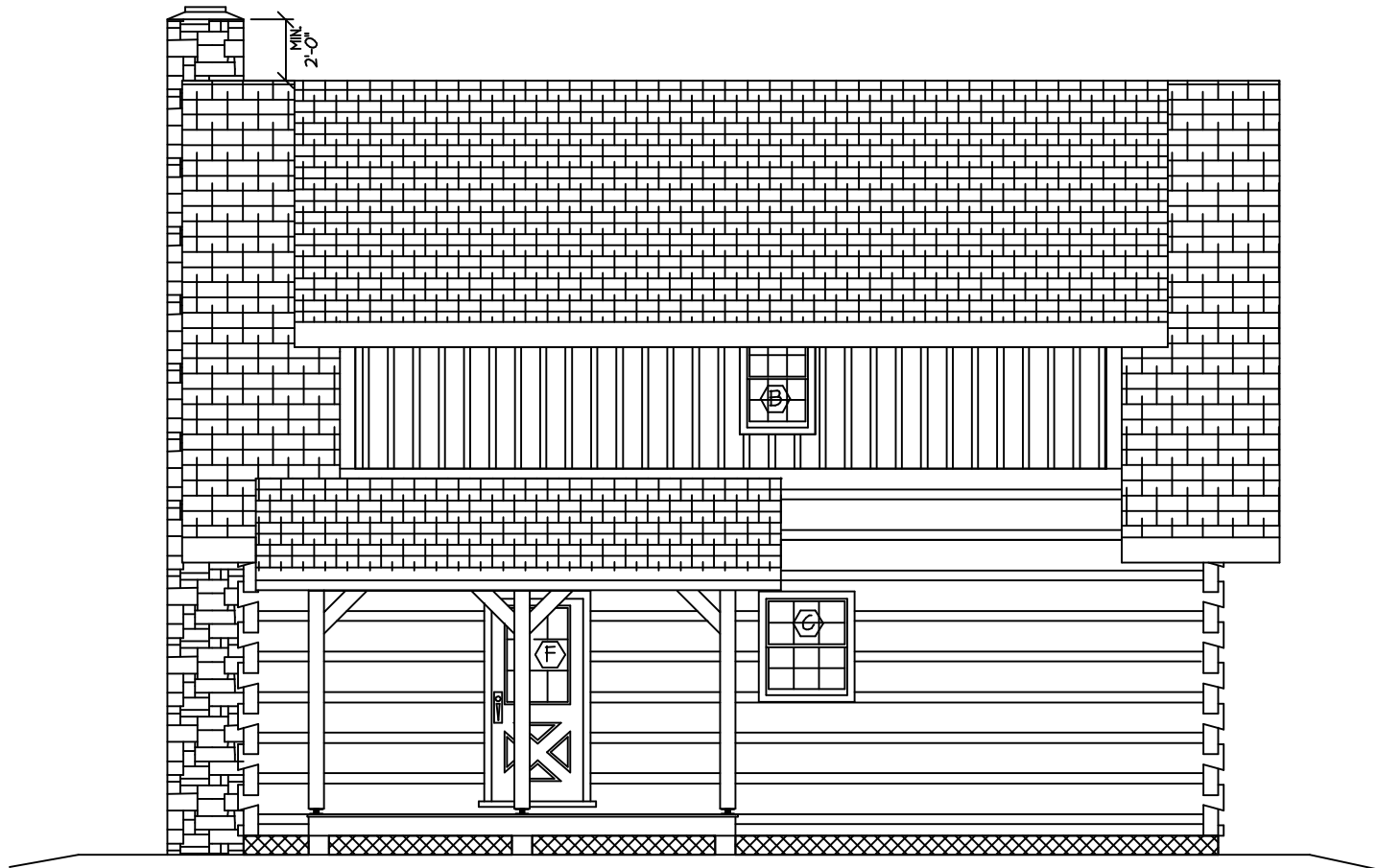
ELEVATION @ REAR
