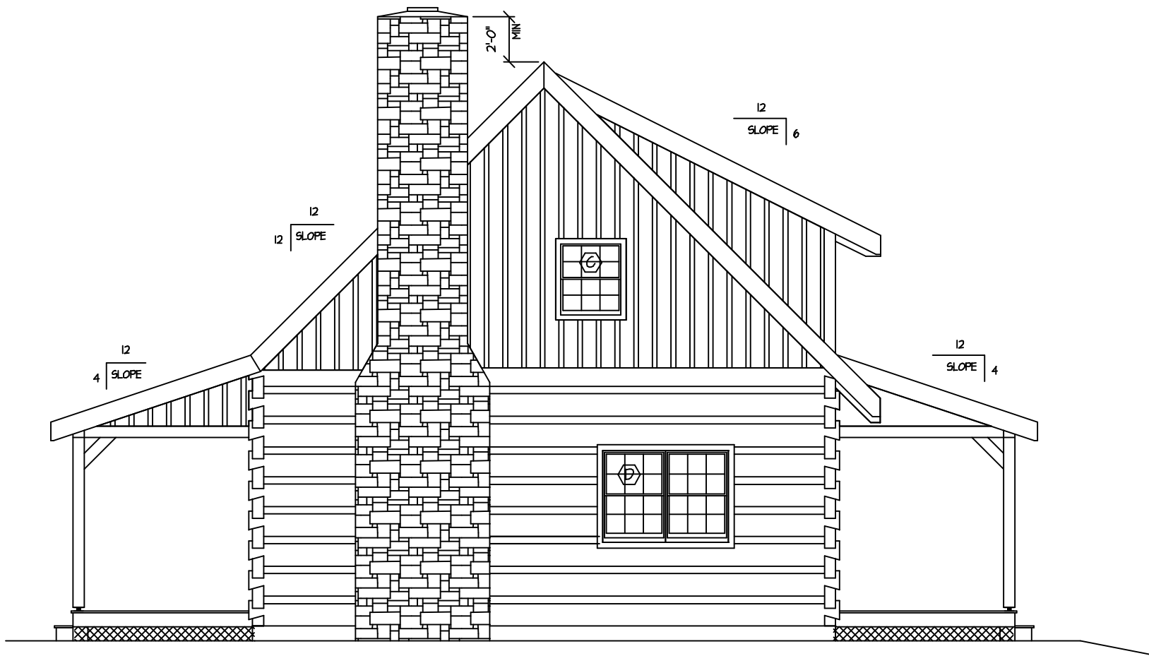
ELEVATION @ RIGHT END
