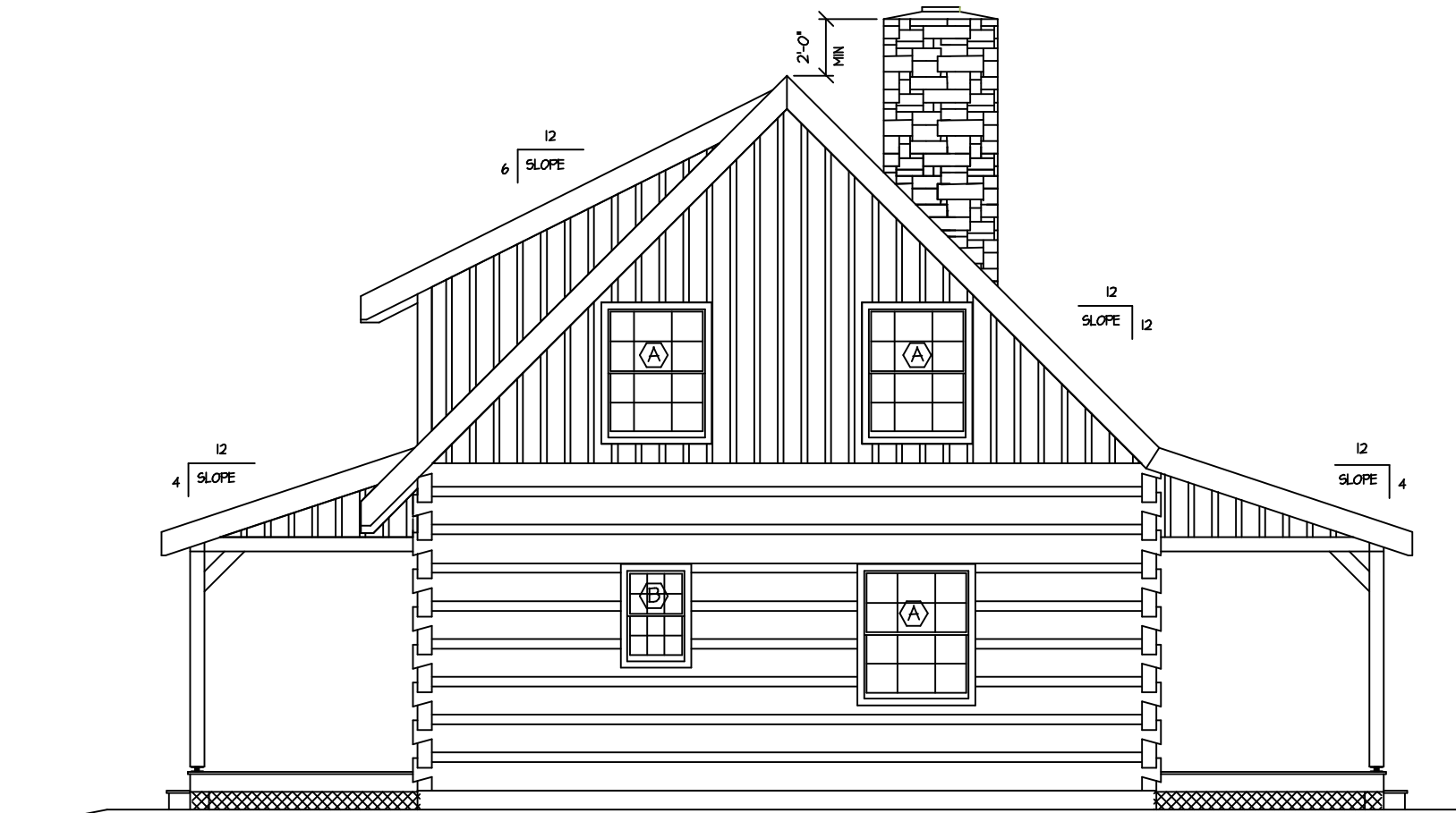
ELEVATION @ LEFT END
