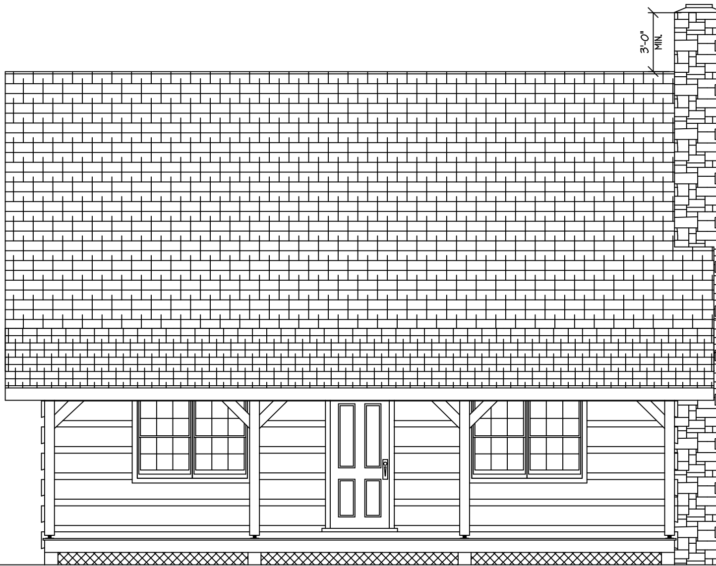
ELEVATION @ FRONT
