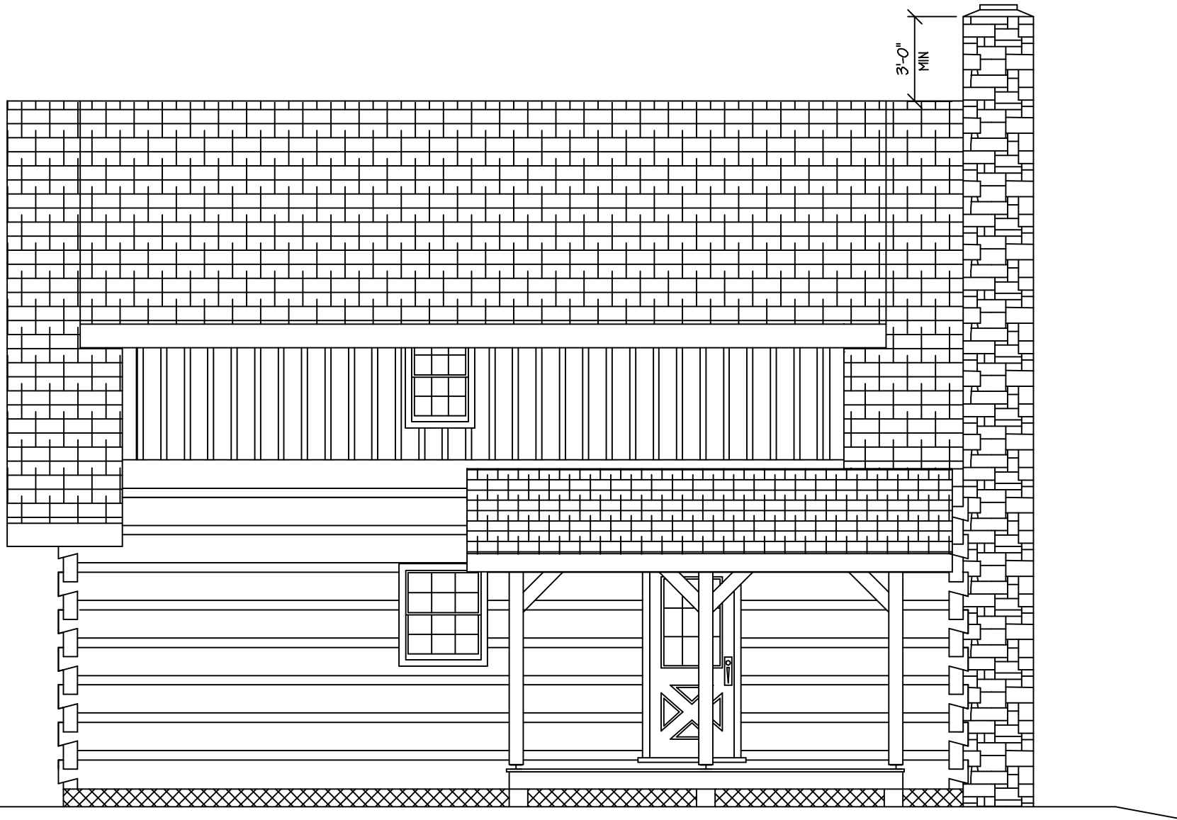
ELEVATION @ REAR
