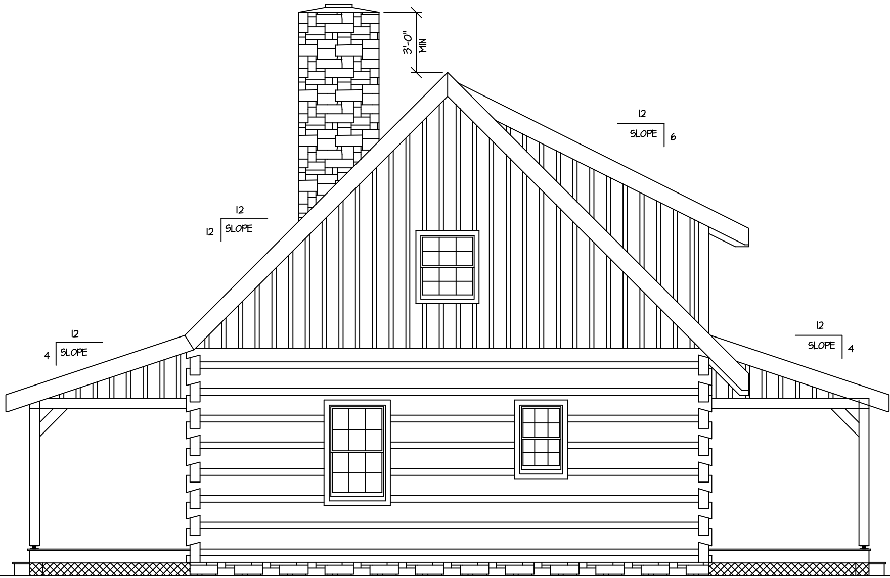
ELEVATION @ RIGHT END
