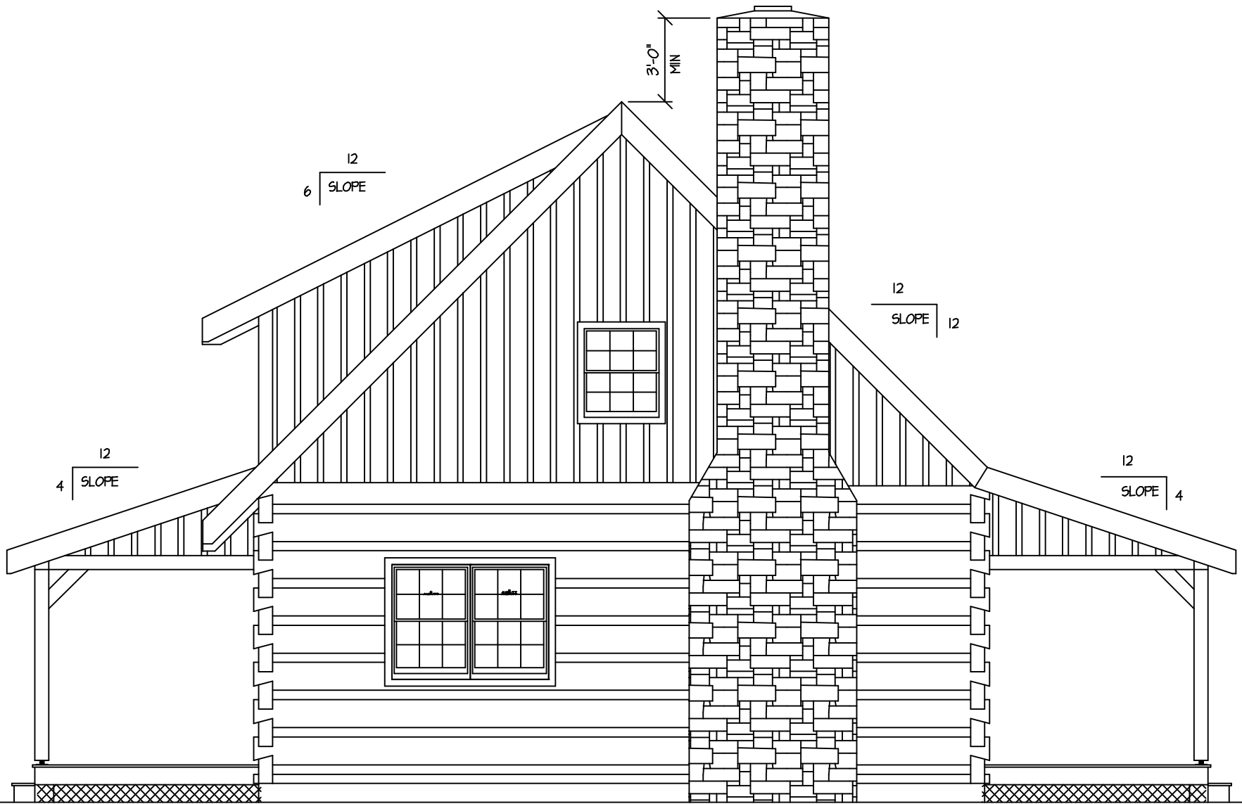
ELEVATION @ LEFT END
