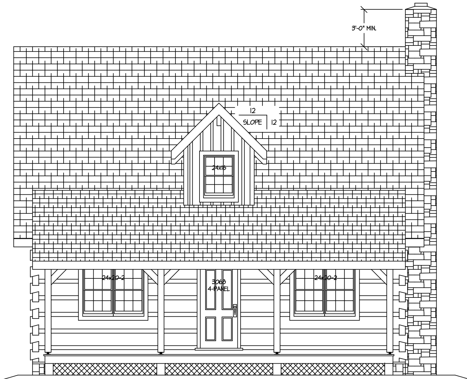
PLAN FRONT
