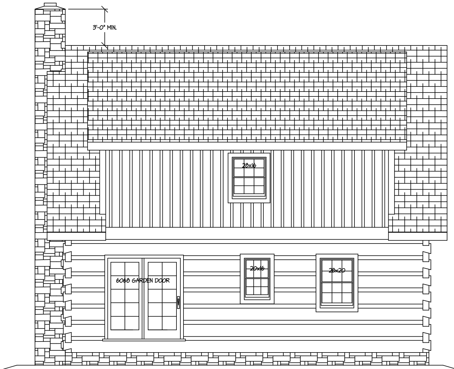
PLAN BACK
