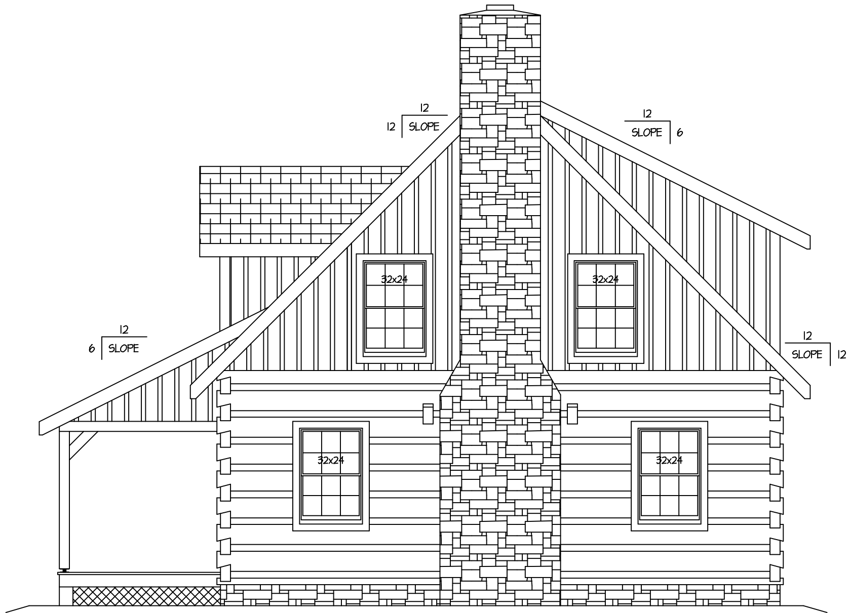
PLAN RIGHT
