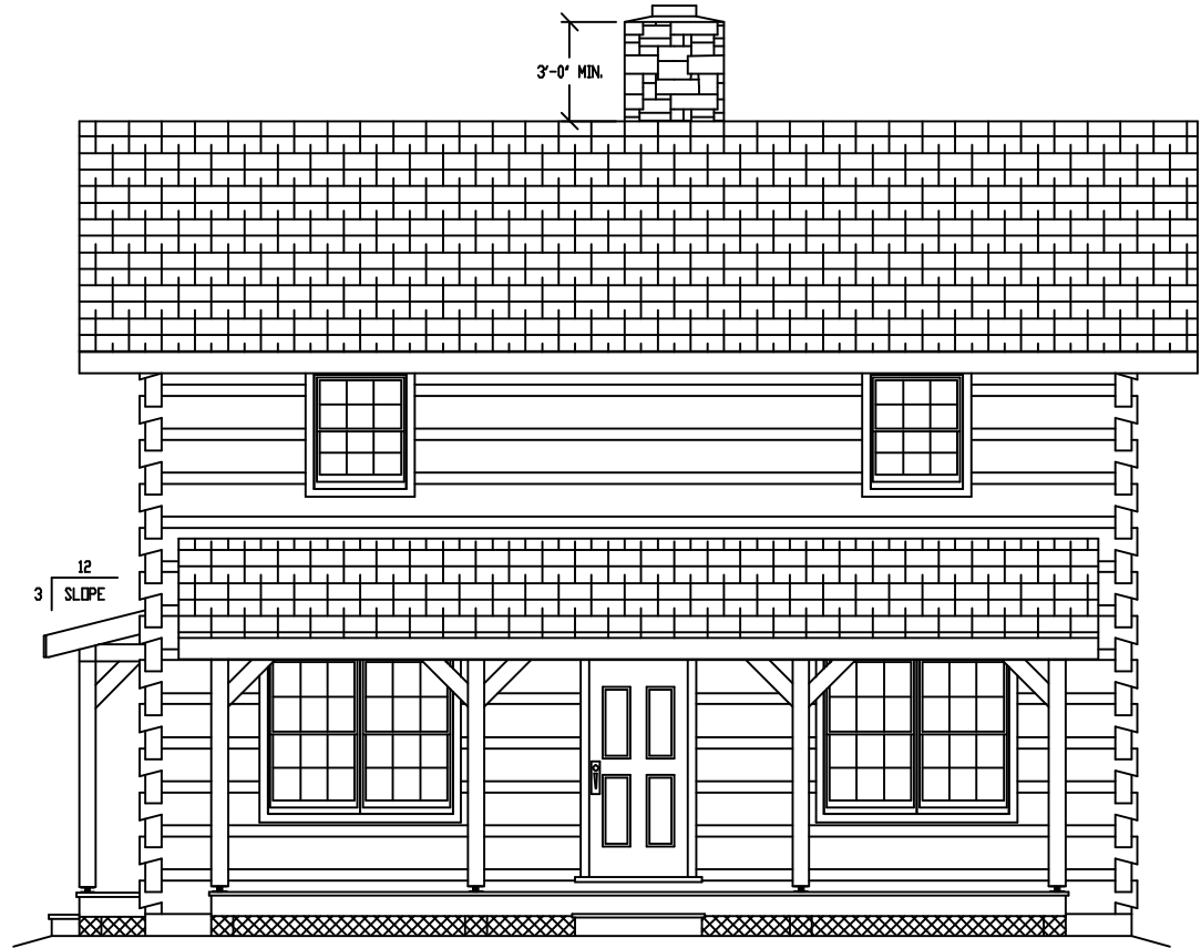
ELEVATION @ FRONT
