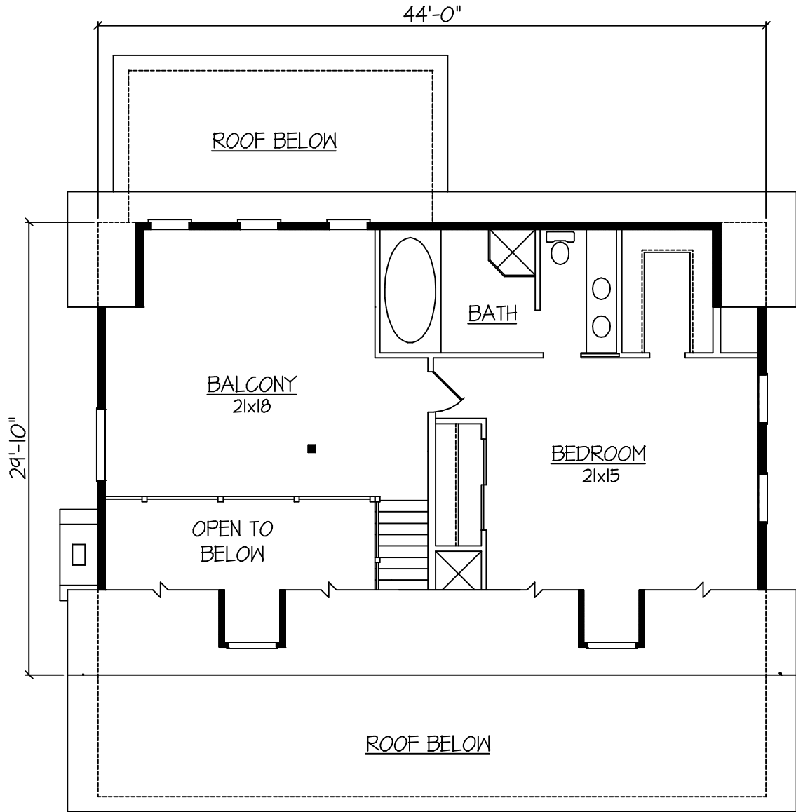
SECOND FLOOR PLAN SECOND FLOOR - 718 SF
