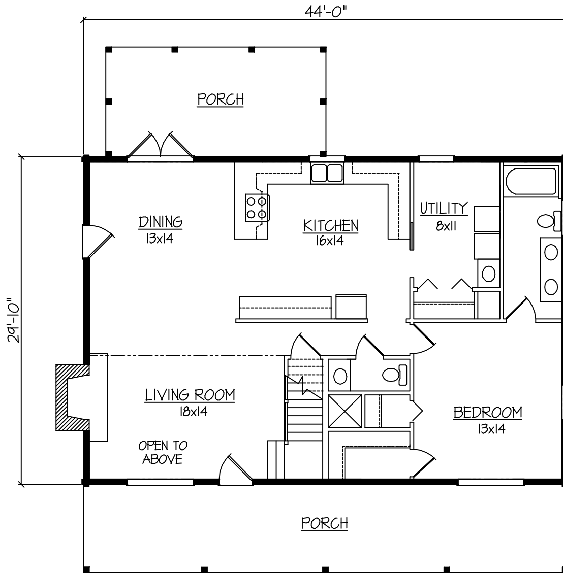
FIRST FLOOR PLAN FIRST FLOOR - 1313 SF TOTAL - 2031 SF
