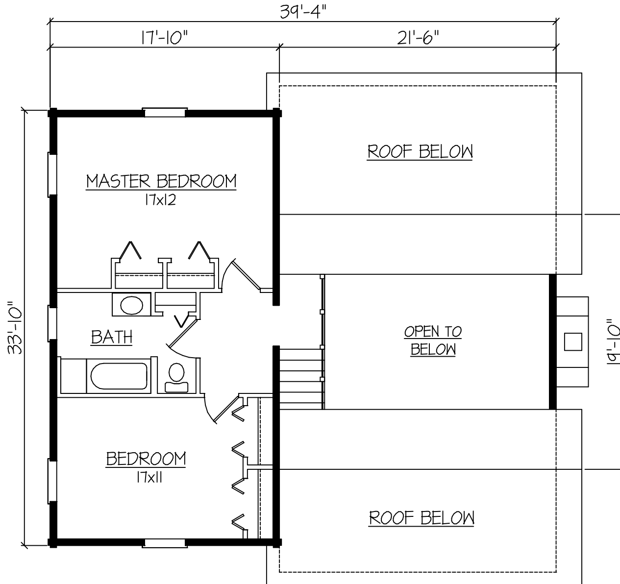
SECOND FLOOR PLAN SECOND FLOOR - 627 SF
