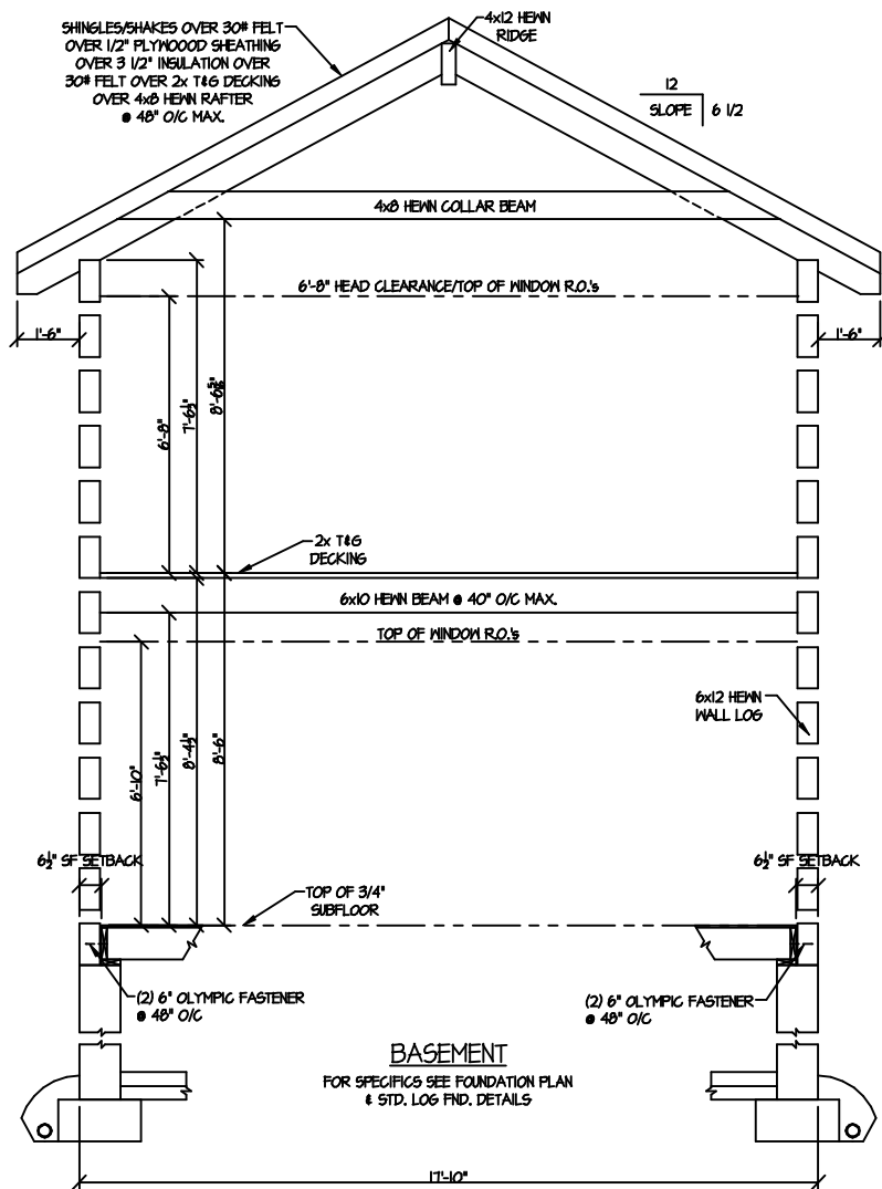
SECTION @ BEDROOMS/KITCHEN/DINING
