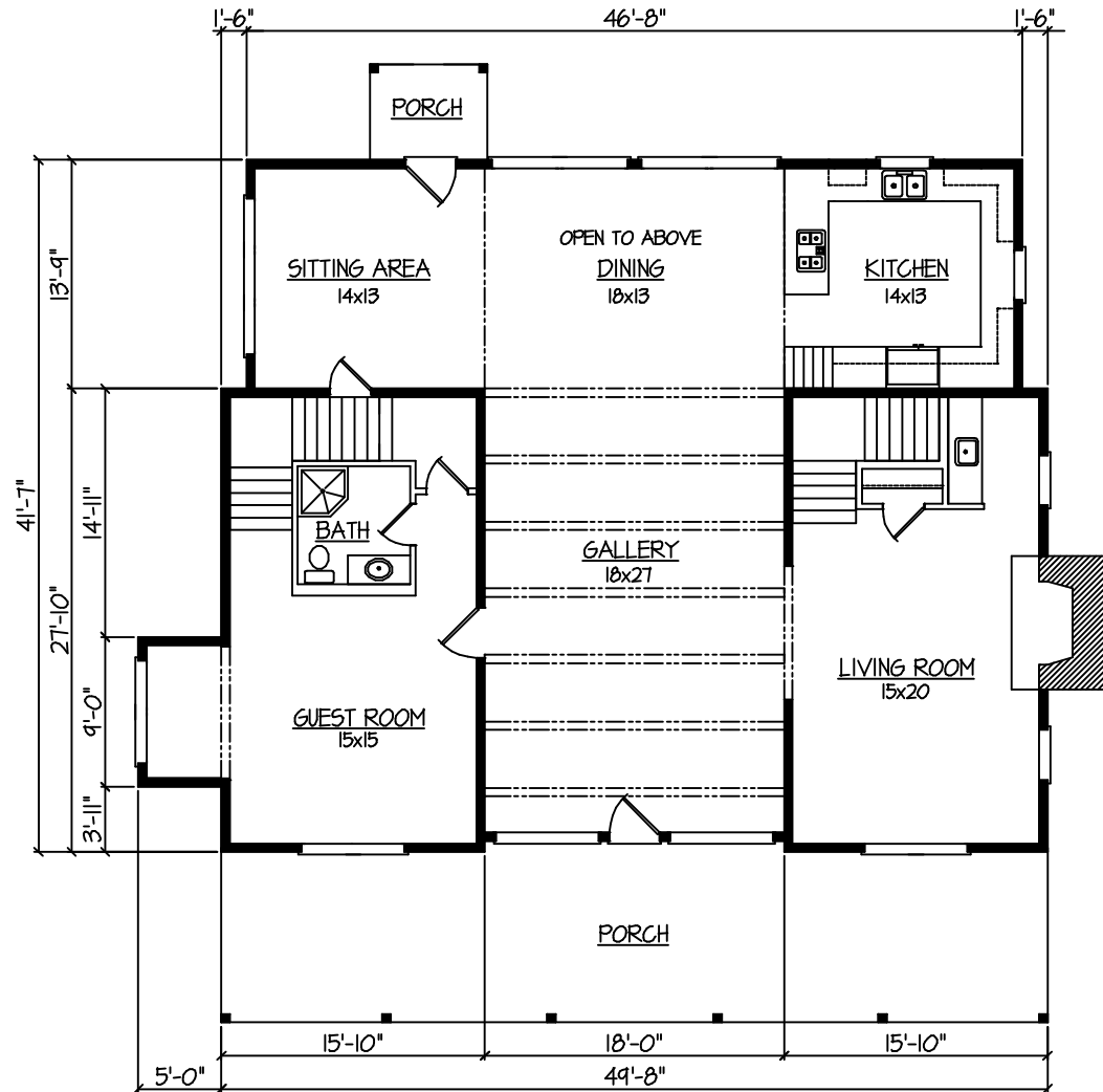
FIRST FLOOR PLAN FIRST FLOOR - 2056 SF TOTAL - 4296 SF
