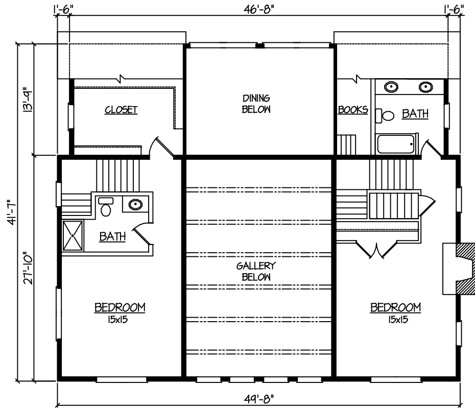
SECOND FLOOR PLAN SECOND FLOOR - 1110 SF
