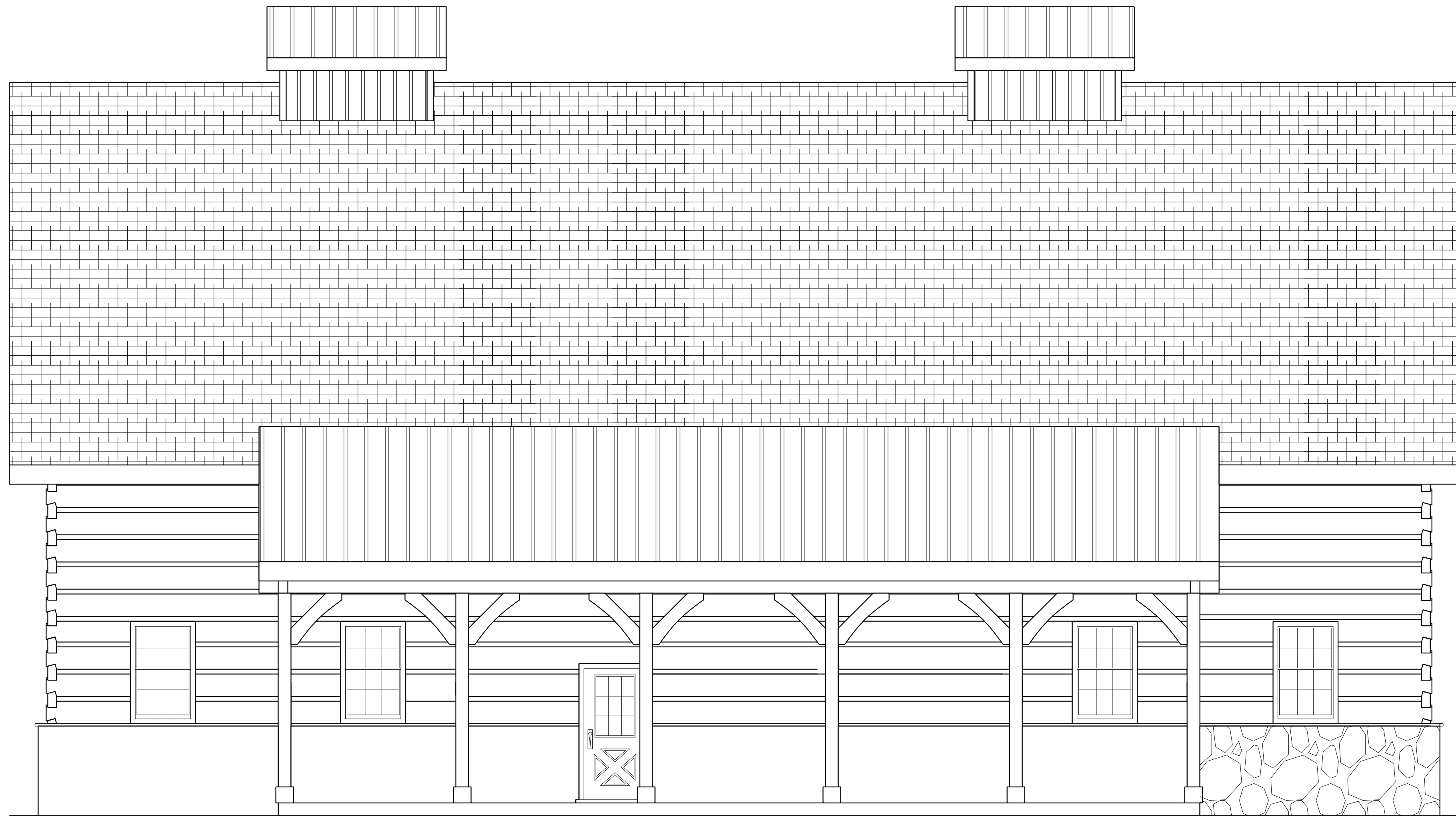
PLAN FRONT ELEVATION
