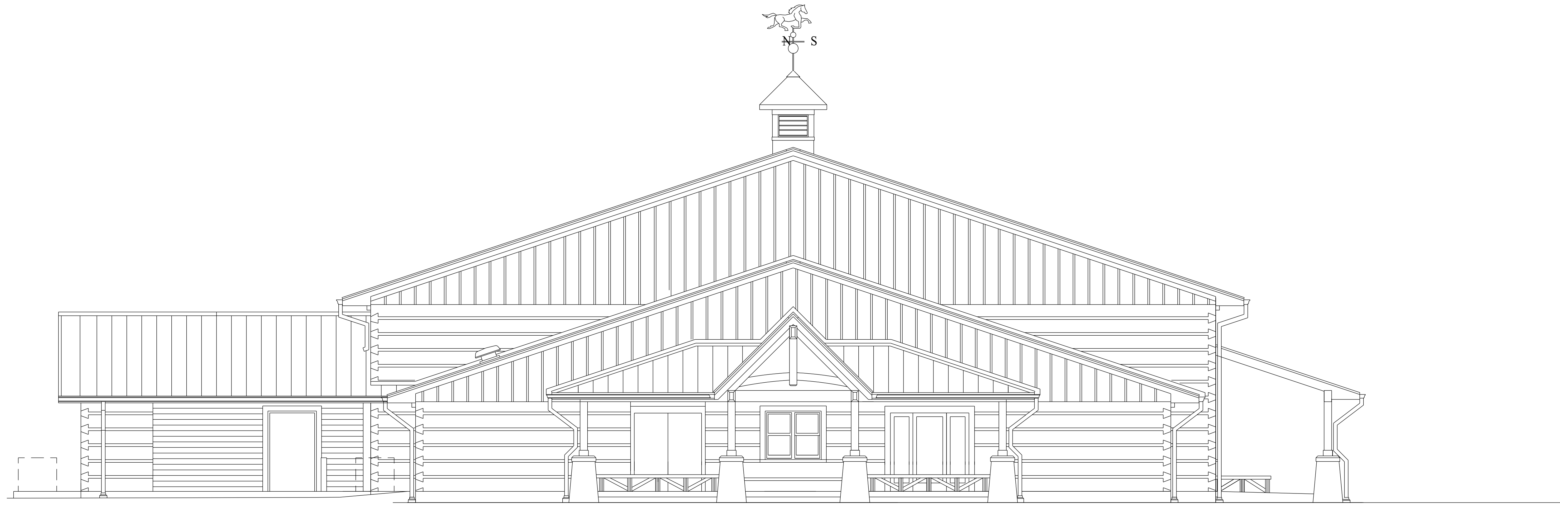
REAR SIDE ELEVATION
